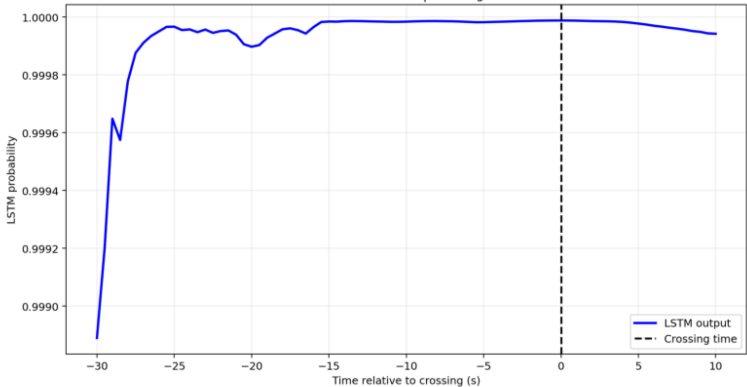
Glitch 1: GPS=1263591424 | crossing at 1059.00 s
