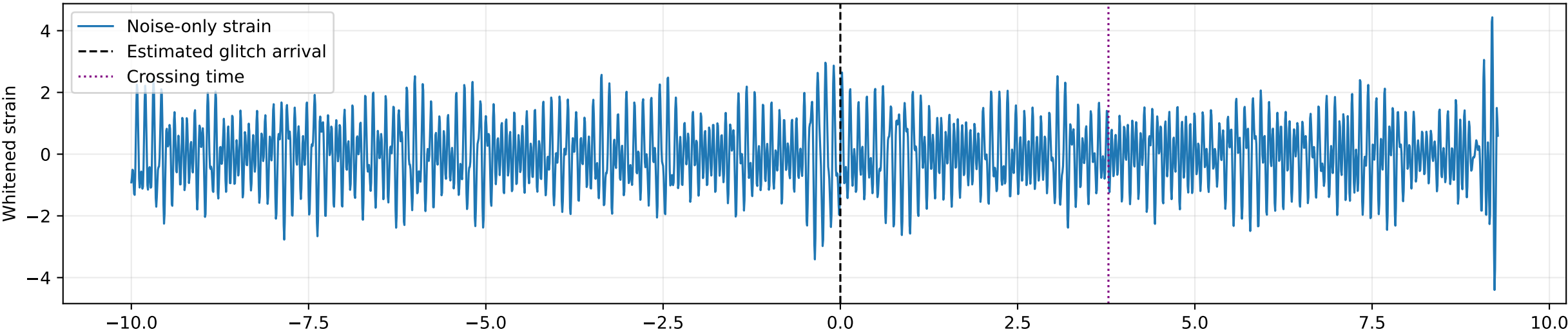
Noise-only glitch candidate | GPS=1263738880 | duration≈39.27s | peak_prob=0.9977
