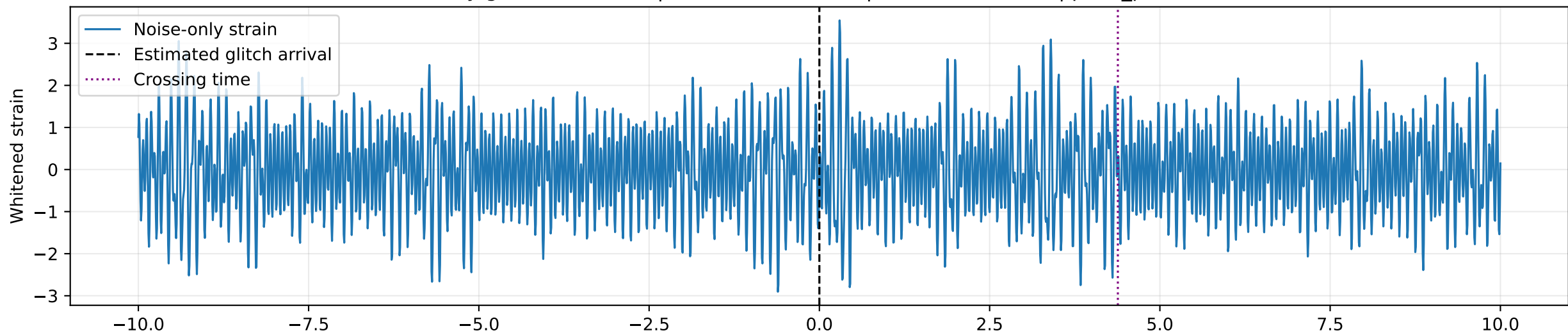
Noise-only glitch candidate | GPS=1263464448 | duration≈39.99s | peak_prob=0.9980
