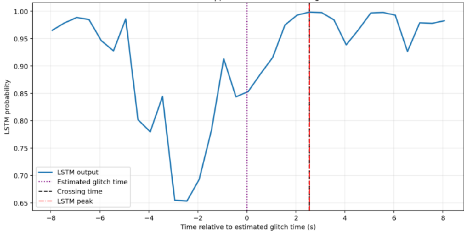
Glitch candidate | GPS=1262575616 cross=2.55 s | peak=2.55 s relative to glitch
