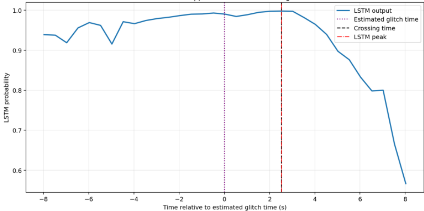
Glitch candidate | GPS=1262997504 cross=2.52 s | peak=2.52 s relative to glitch
