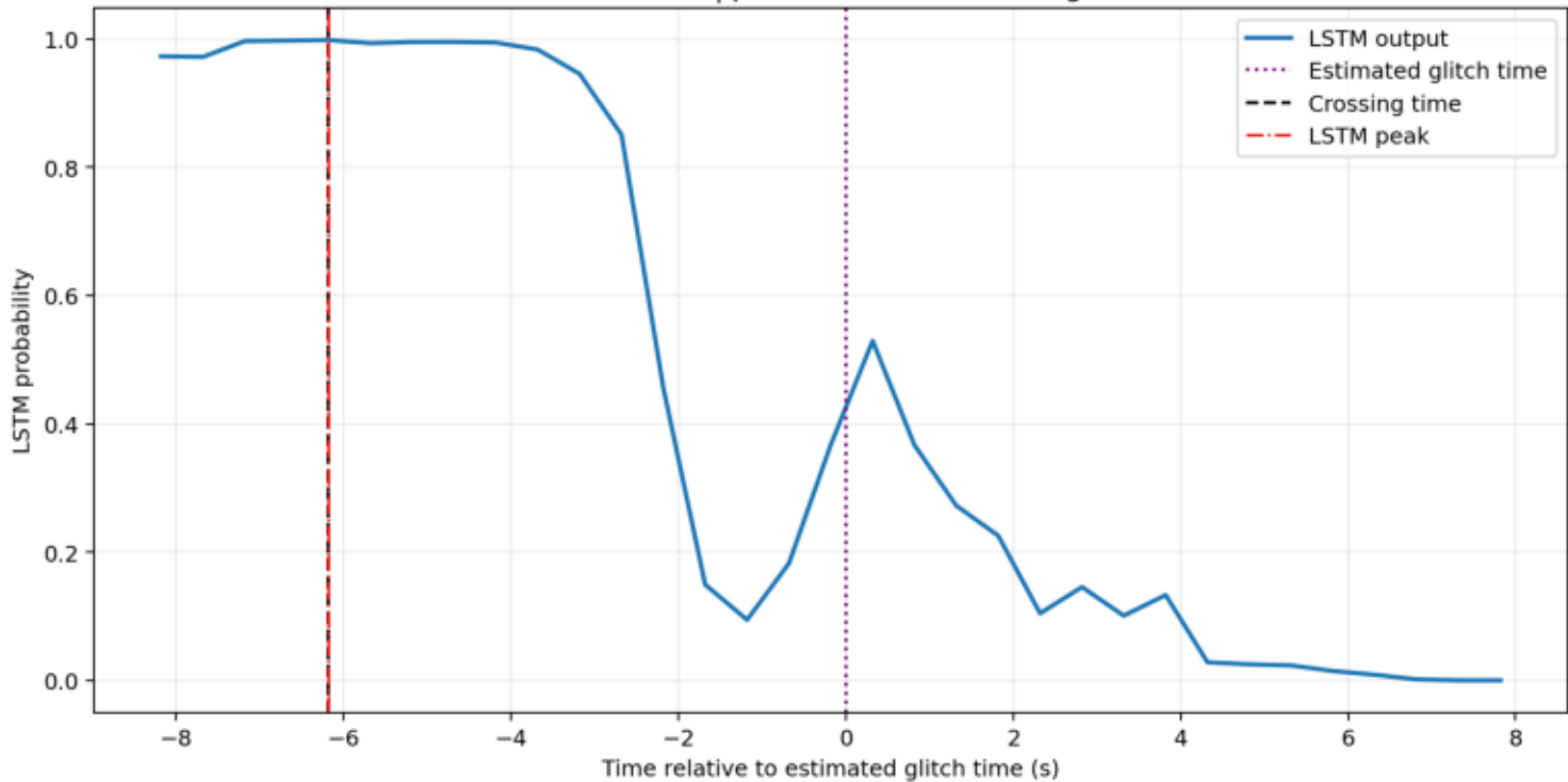
Glitch candidate | GPS=1262575616 cross=-6.18 s | peak=-6.18 s relative to glitch
