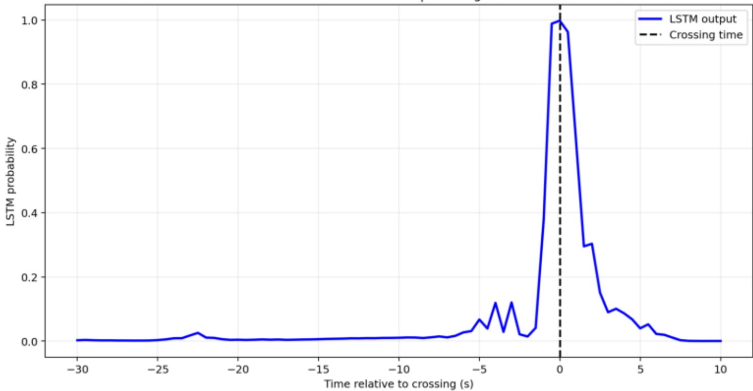
Glitch 14: GPS=1264181248 | crossing at 3344.00 s
