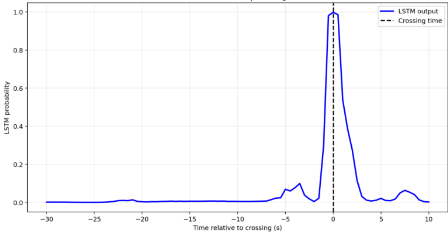
Glitch 12: GPS=1263599616 | crossing at 1270.00 s
