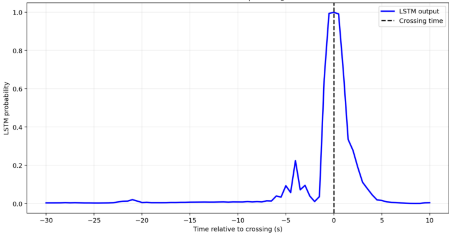
Glitch 8: GPS=1263108096 | crossing at 2955.50 s
