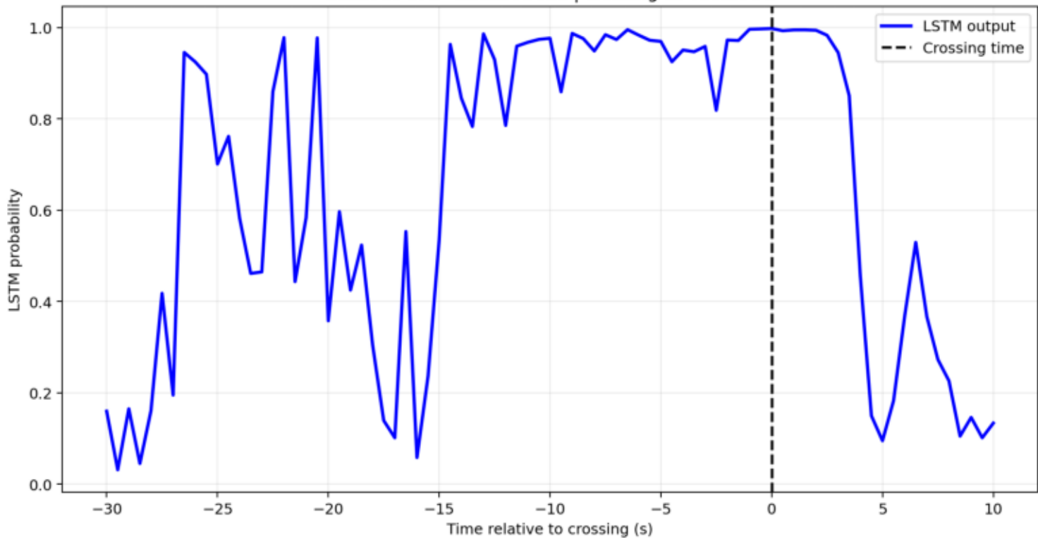
Glitch 5: GPS=1262575616 | crossing at 4002.00 s
