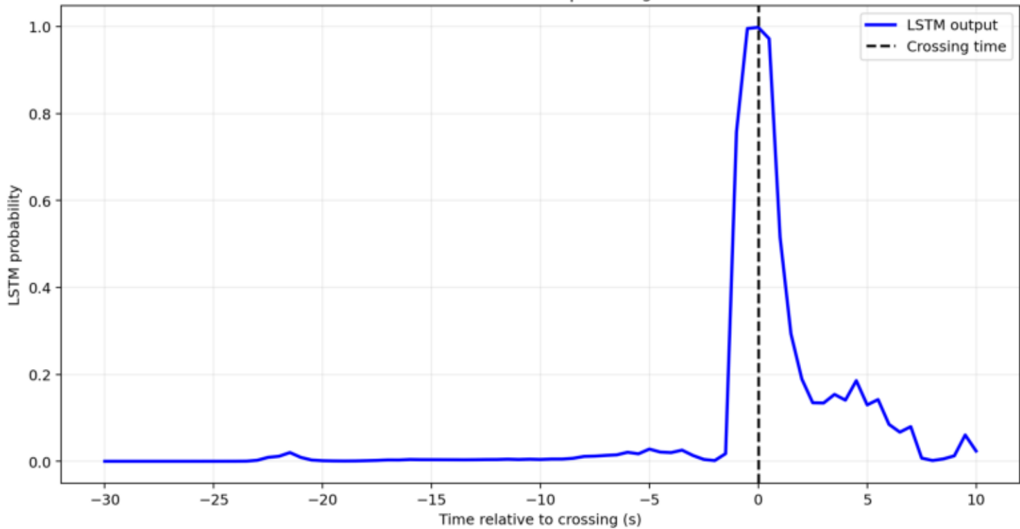
Glitch 13: GPS=1264062464 | crossing at 1371.00 s
