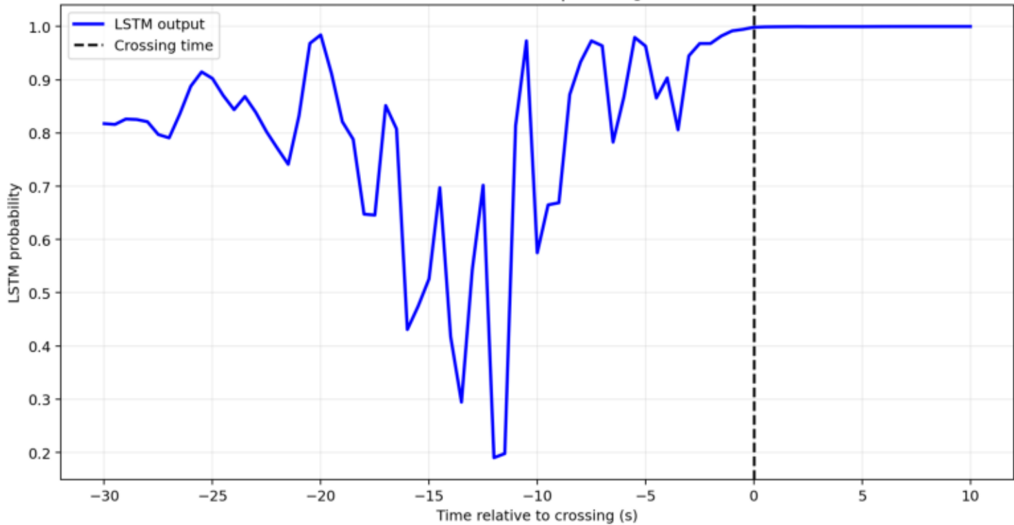
Glitch 4: GPS=1262575616 | crossing at 2533.00 s
