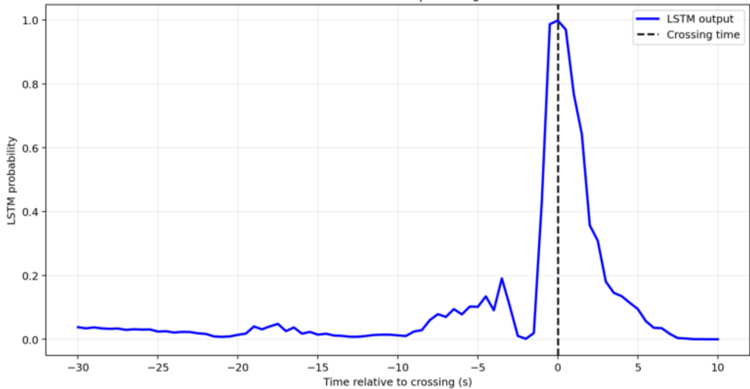
Glitch 11: GPS=1263464448 | crossing at 3467.50 s
