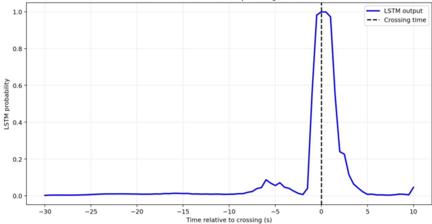
Glitch 16: GPS=1264422912 | crossing at 3621.50 s
