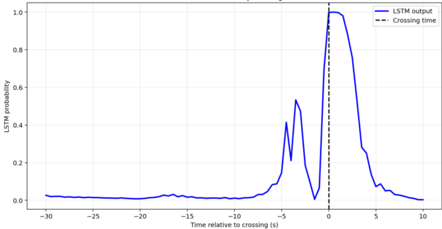
Glitch 15: GPS=1264365568 | crossing at 2197.50 s
