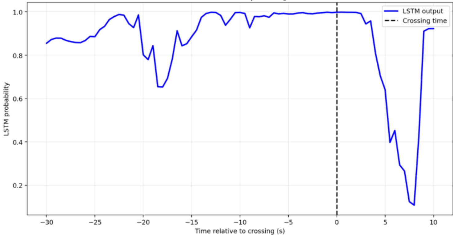
Glitch 3: GPS=1262575616 | crossing at 1054.00 s
