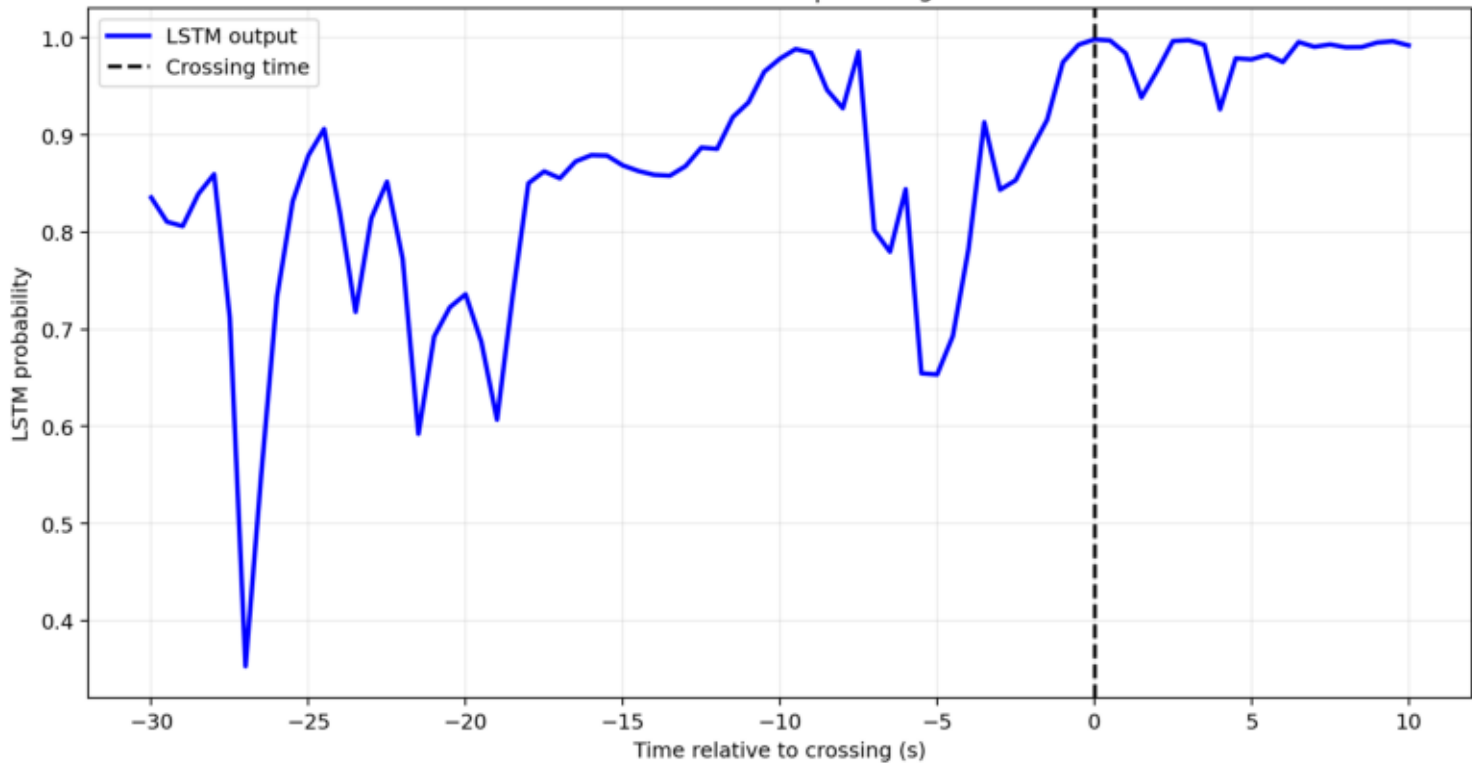
Glitch 1: GPS=1262575616 | crossing at 1041.00 s
