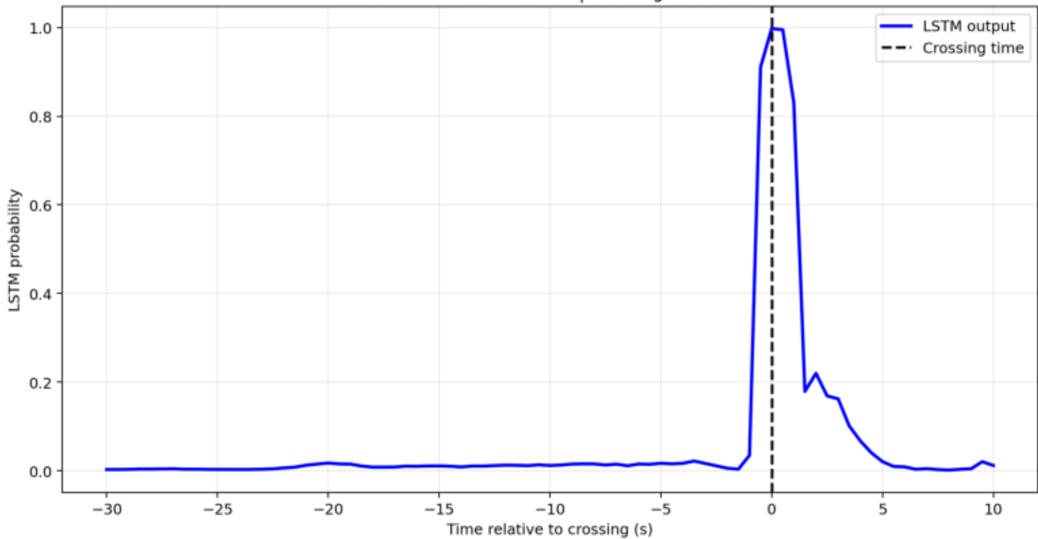
Glitch 17: GPS=1264615424 | crossing at 1436.50 s
