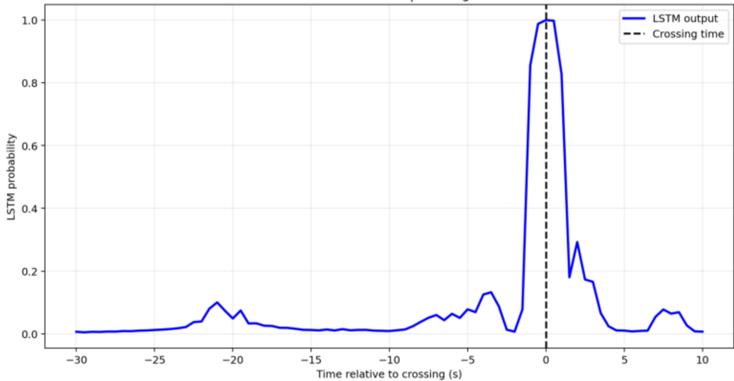
Glitch 10: GPS=1263345664 | crossing at 3276.50 s
