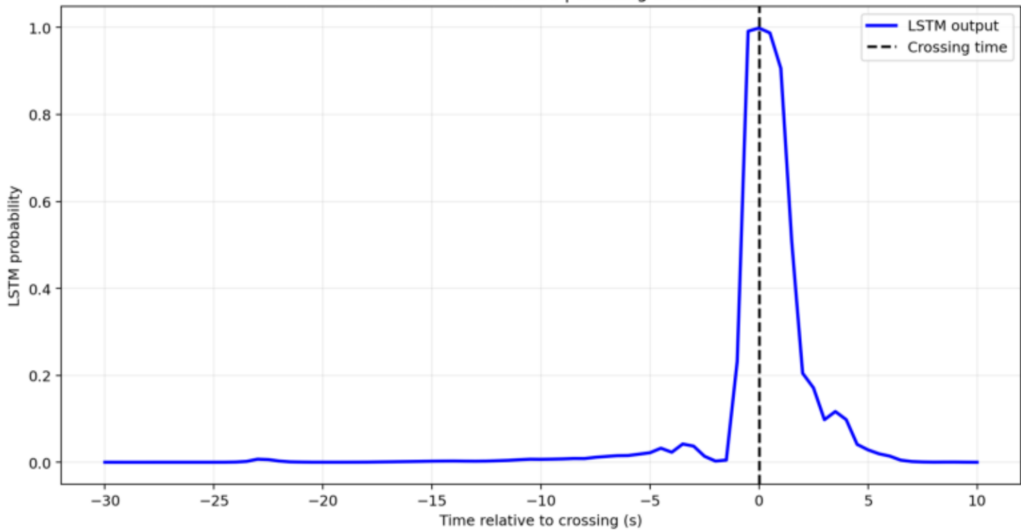
Glitch 6: GPS=1262792704 | crossing at 1542.50 s
