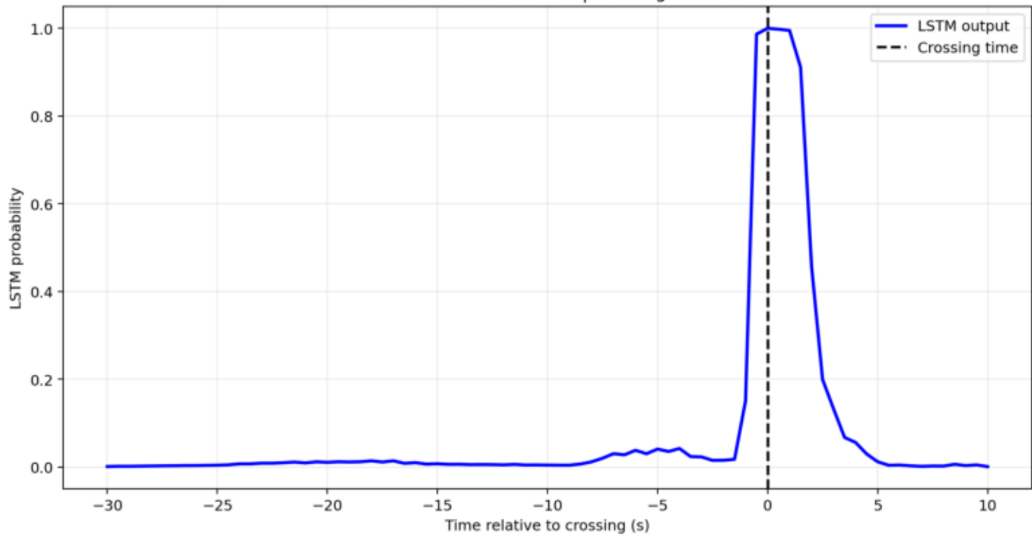
Glitch 18: GPS=1264627712 | crossing at 317.50 s
