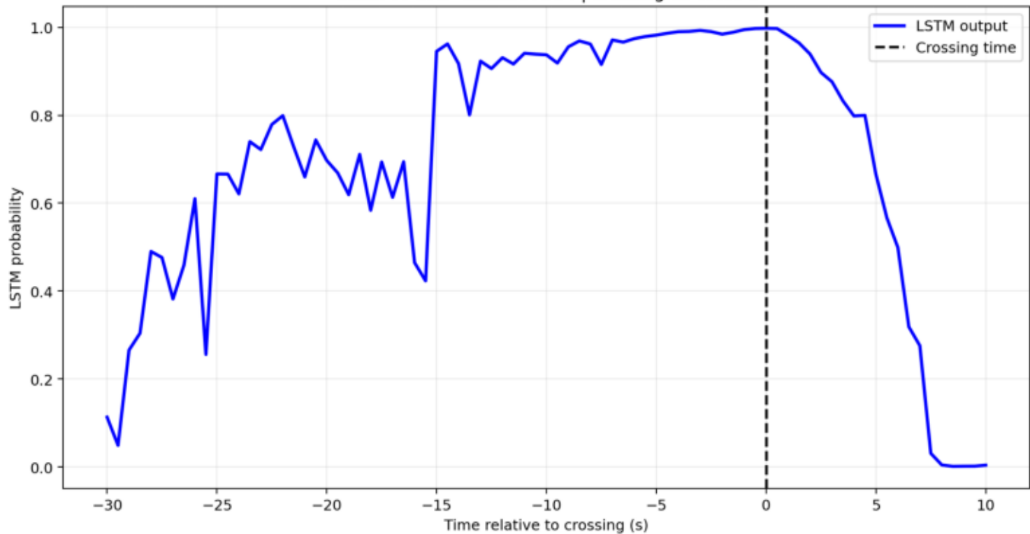
Glitch 7: GPS=1262997504 | crossing at 47.00 s
