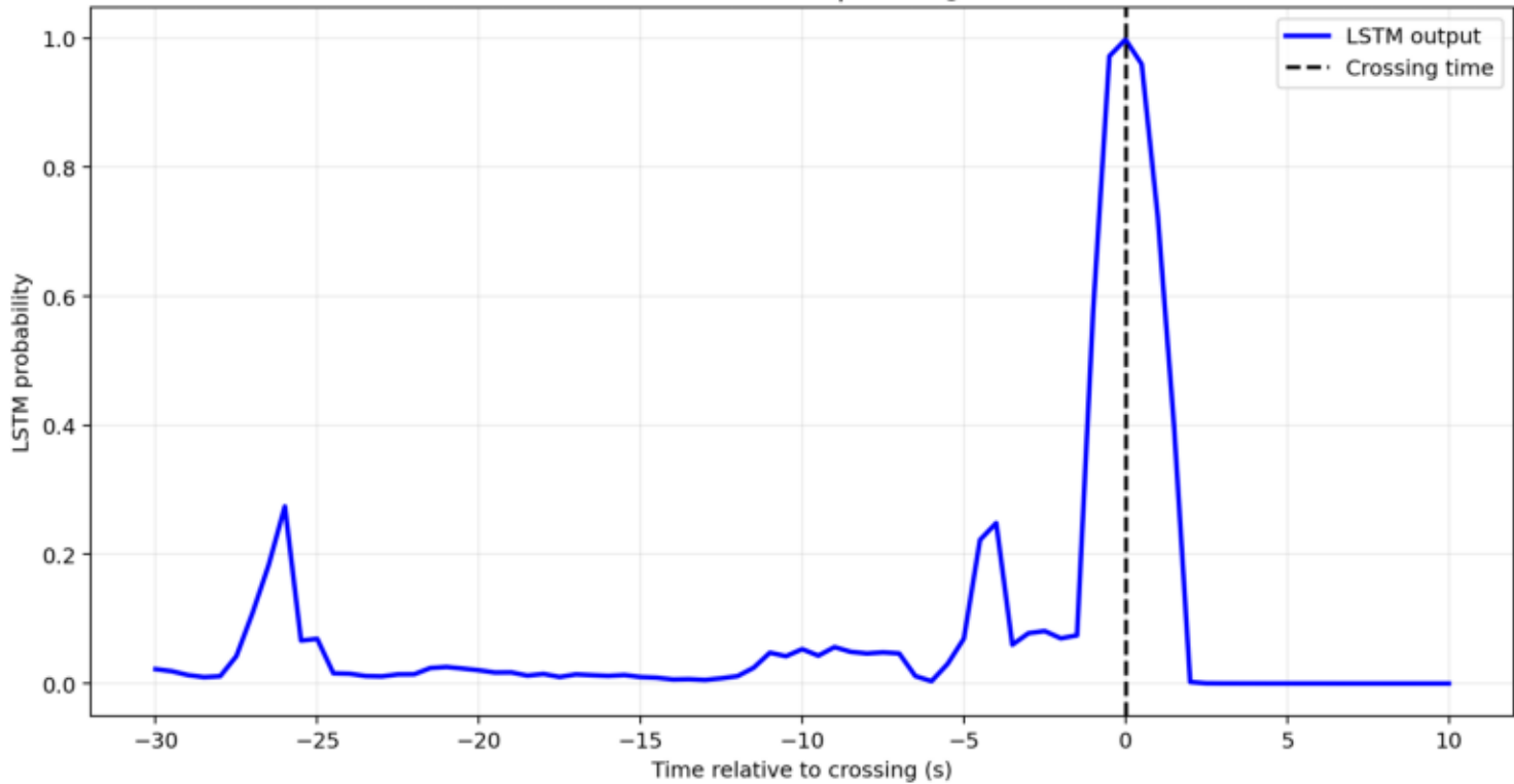
Glitch 9: GPS=1263190016 | crossing at 1837.50 s
