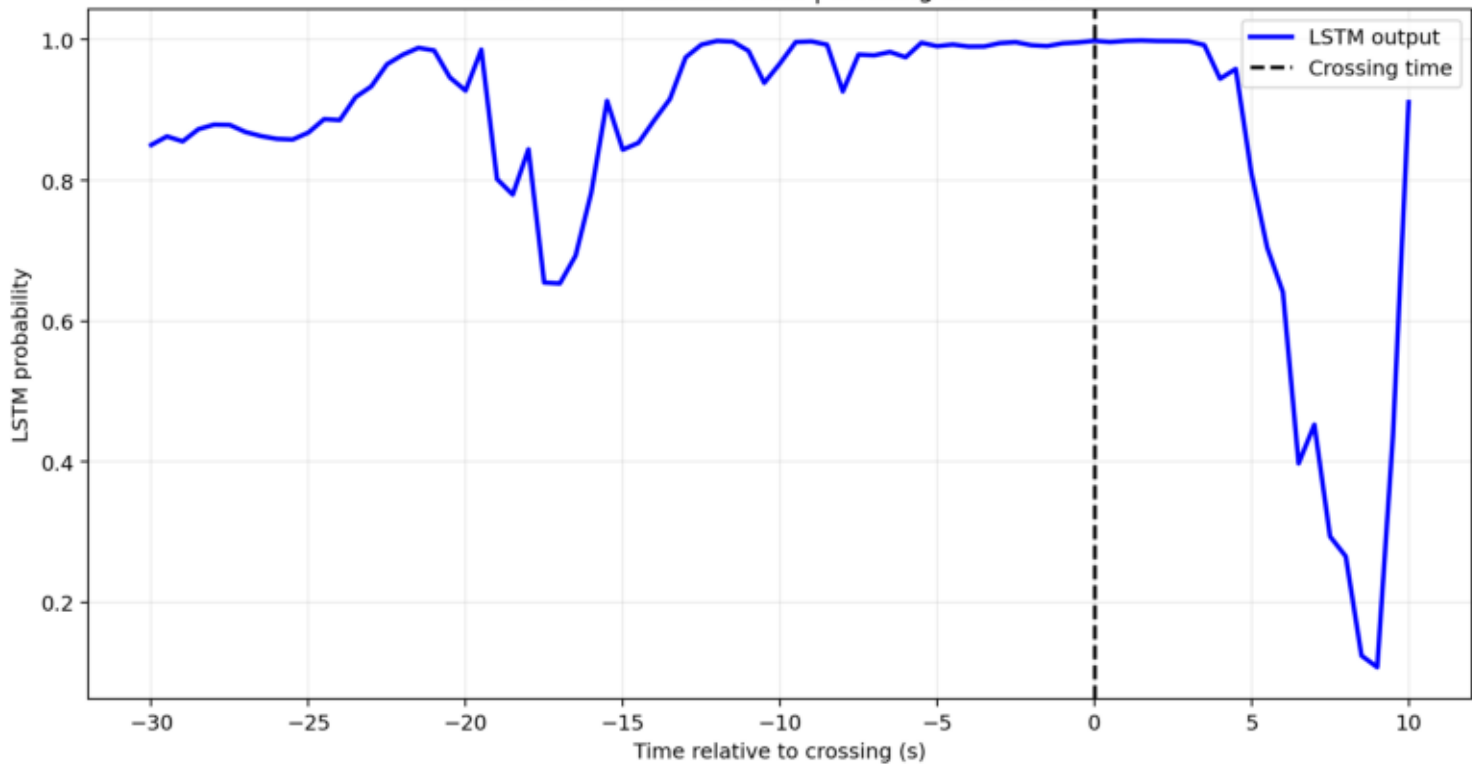
Glitch 2: GPS=1262575616 | crossing at 1053.00 s
