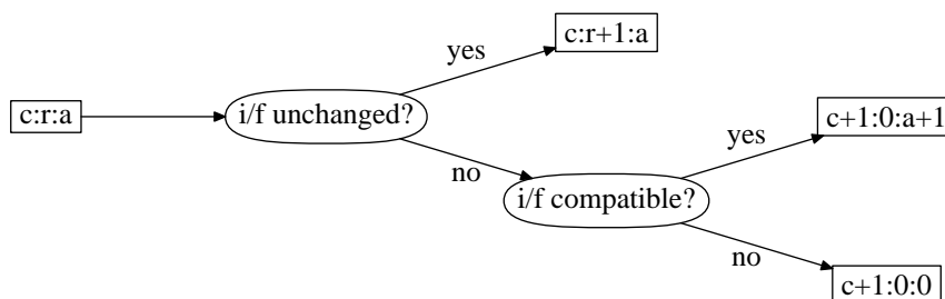
Figure 5: Updating -version-info specifications
