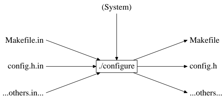
Figure 3: Inputs and outputs to configure
