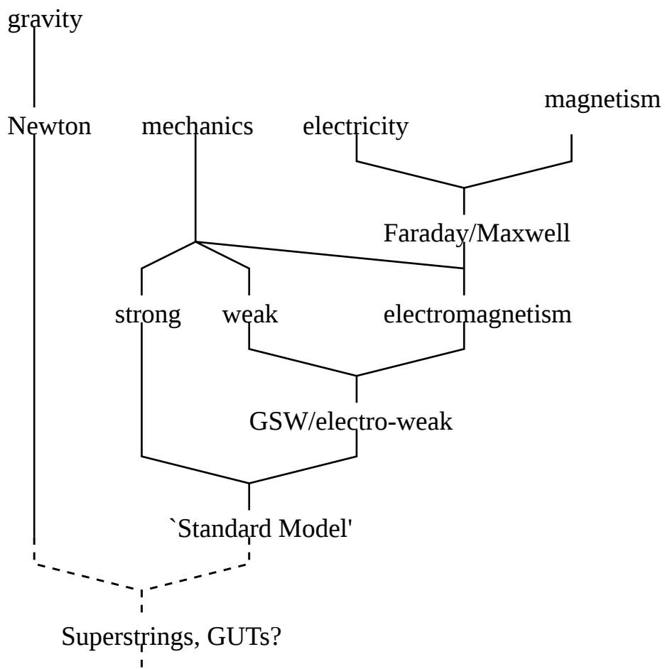
Figure 3: Historically, successive forces have been unified into, potentially, a single force.
