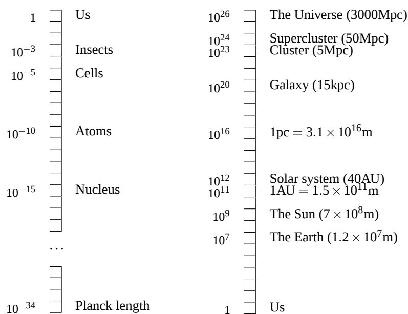
Figure 2: Size scales in the universe
