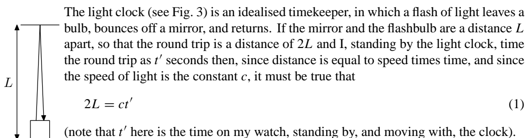
Figure 3: The light clock
