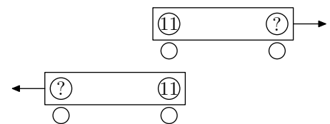
Figure 2: The trains, a little later.
