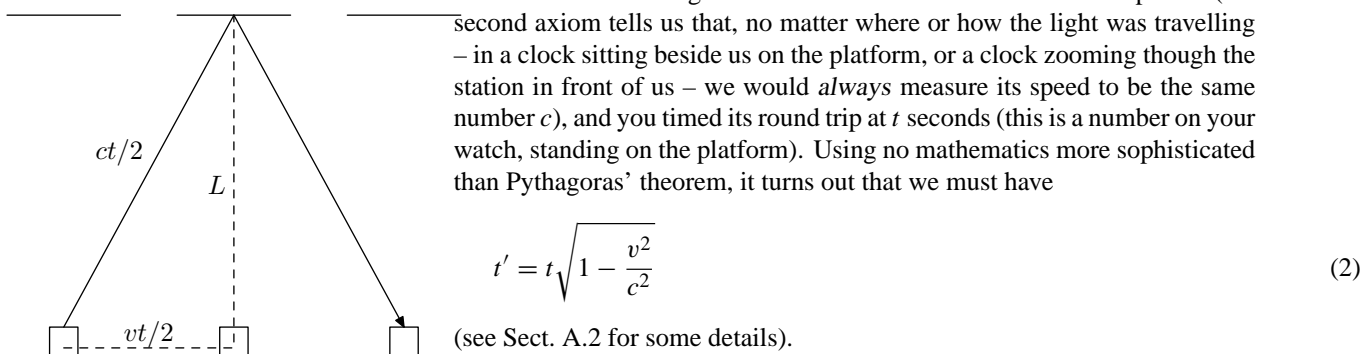
Figure 4: The light clock, as it's perceived when it's moving past you.
