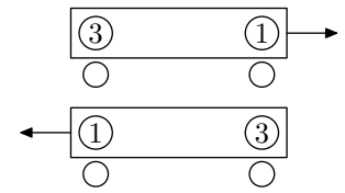
Figure 1: Trains passing in the night.
