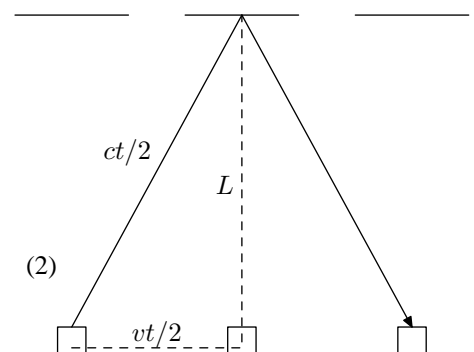
Figure 4: The light clock, as it's perceived when it's moving past you.
