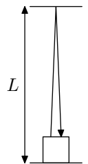
Figure 3: The light clock
