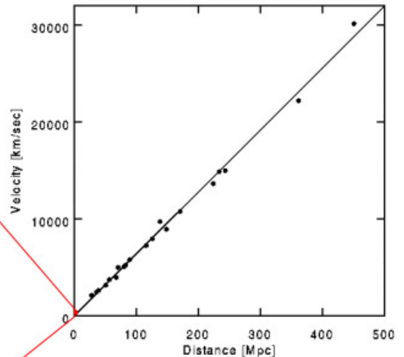
recent SN1a data
