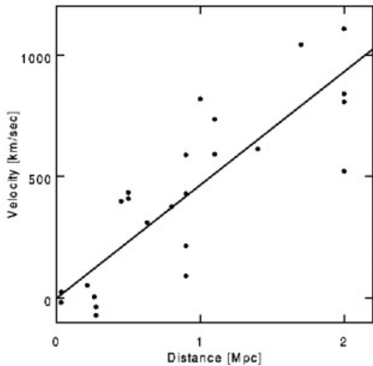
Hubble's 1929 data
