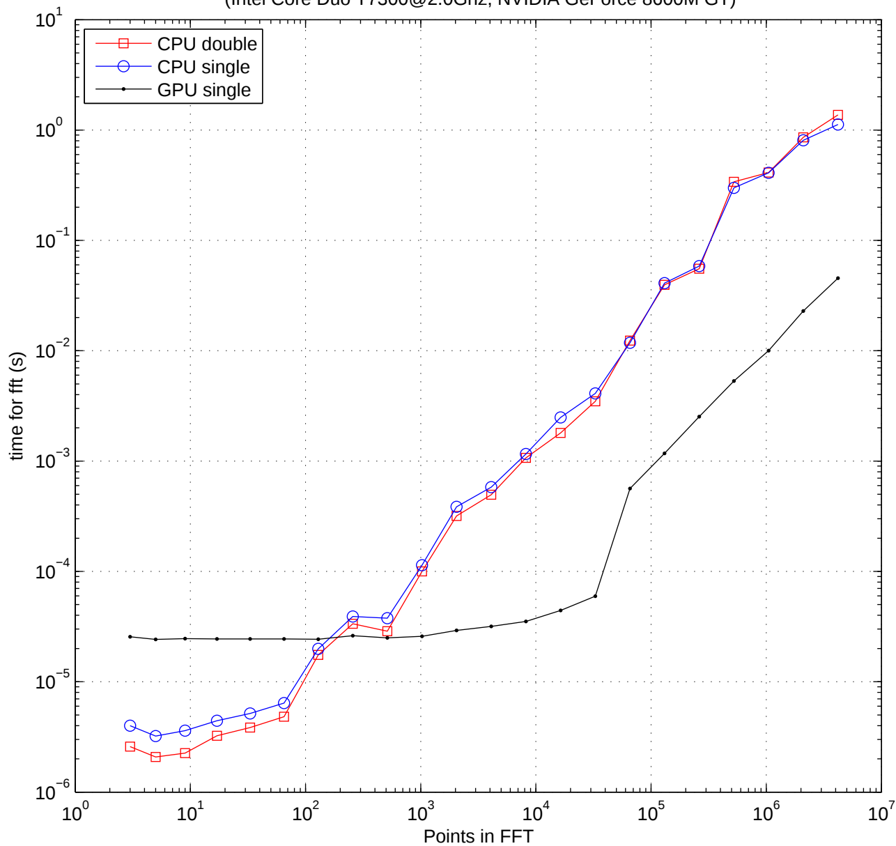
GPU vs. CPU speedup for FFTs of (2^n+1) points (Intel Core Duo T7300@2.0Ghz, NVIDIA GeForce 8600M GT)
