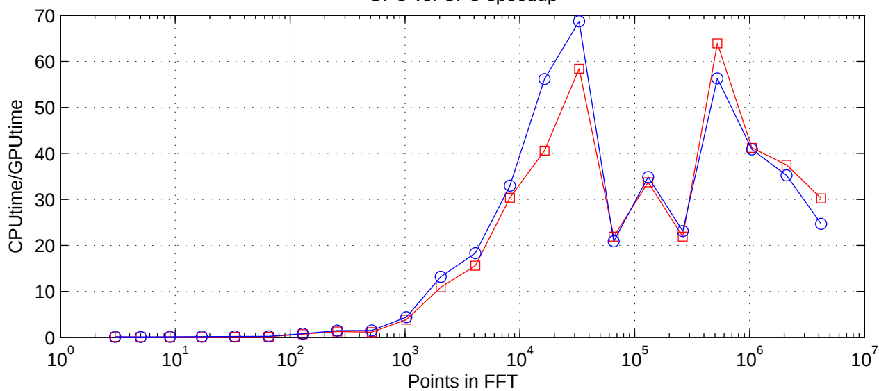
GPU vs. CPU speedup
