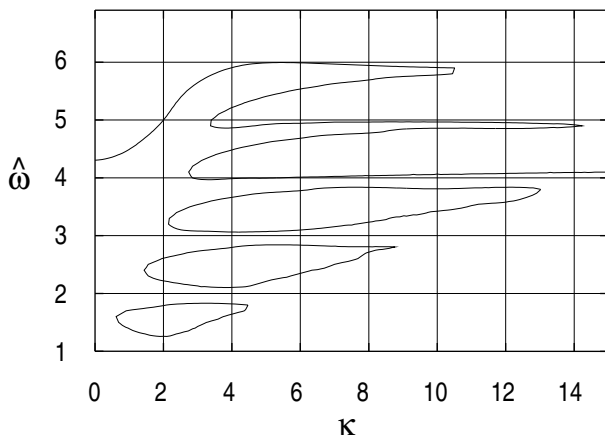
FIG. 4: Dispersion curves showing solutions in \hat{\omega} - \kappa space for the case a = 20 , \hat{\omega}_p = 3 . Vertical axis is \hat{\omega} ; horizontal axis is \kappa .
