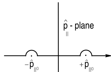
FIG. 7: The Bromwich contour for the \hat{p}_{\parallel} integration
