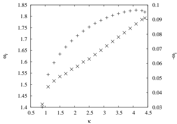
FIG. 2: Pluses (+) show the upper loop of the dispersion curve \hat{\omega}_r (left y-axis) versus \kappa (x-axis) for a = 10 , and 1 < \hat{\omega}_r < 2 . The crosses ( \times ) show how -\hat{\omega}_i (right y-axis) varies as a function of \kappa along the dispersion curve.
