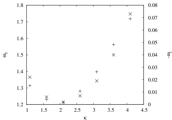
FIG. 3: Caption as for Fig. 2, showing the real and imaginary parts on the lower loop of the same dispersion curve.
