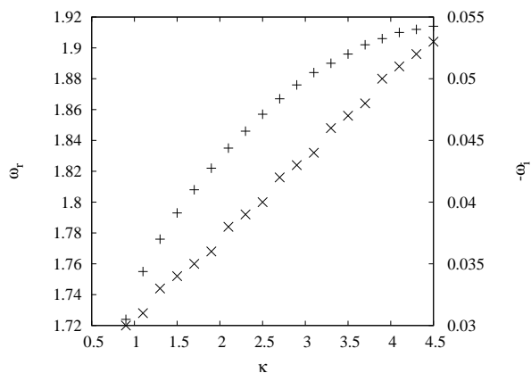
FIG. 4: Pluses (+) show the upper loop of the dispersion curve \hat{\omega}_r (left y-axis) versus \kappa (x-axis) for a = 20 , and 1 < \hat{\omega}_r < 2 . The crosses ( \times ) show how -\hat{\omega}_i (right y-axis) varies as a function of \kappa along the dispersion curve.
