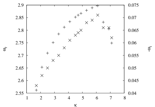
FIG. 6: Pluses (+) show the upper loop of the dispersion curve \hat{\omega}_r (left y-axis) versus \kappa (x-axis) for a = 20 , and 2 < \hat{\omega}_r < 3 . The crosses ( \times ) show how -\hat{\omega}_i (right y-axis) varies as a function of \kappa along the dispersion curve.
