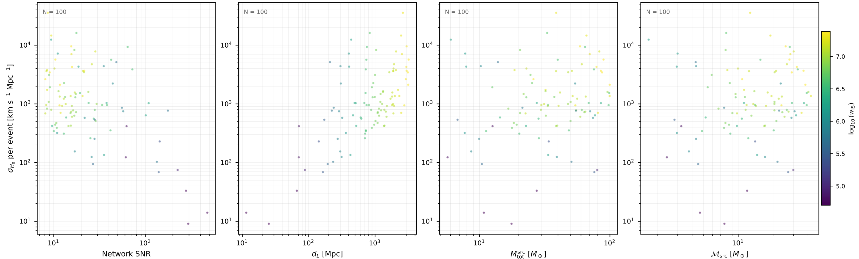
Fisher \sigma_{H_0} per event aLIGO_HLV / var03 (100 events, 10 seed(s))
