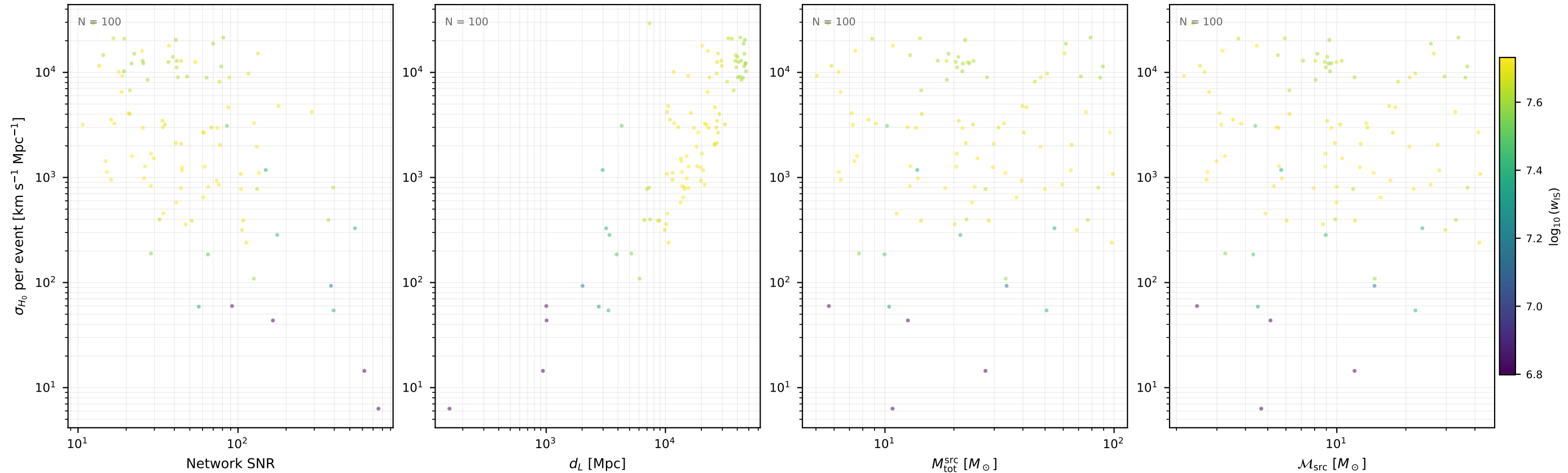
Fisher \sigma_{H_0} per event ET_CE / var07 (100 events, 10 seed(s))
