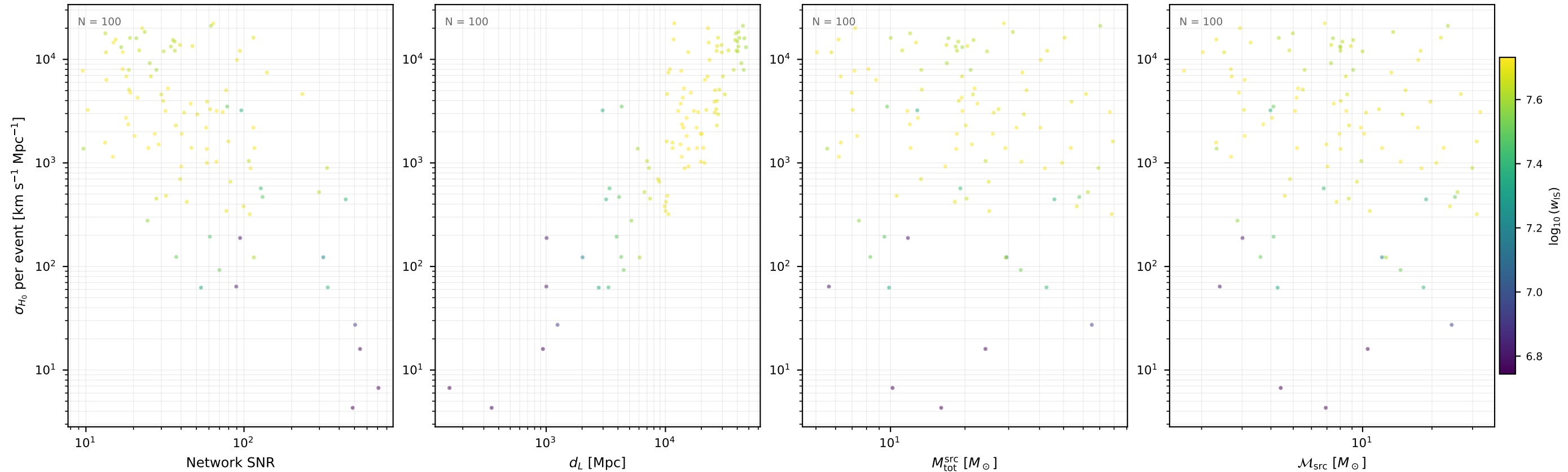
Fisher \sigma_{H_0} per event ET_CE / var06 (100 events, 10 seed(s))
