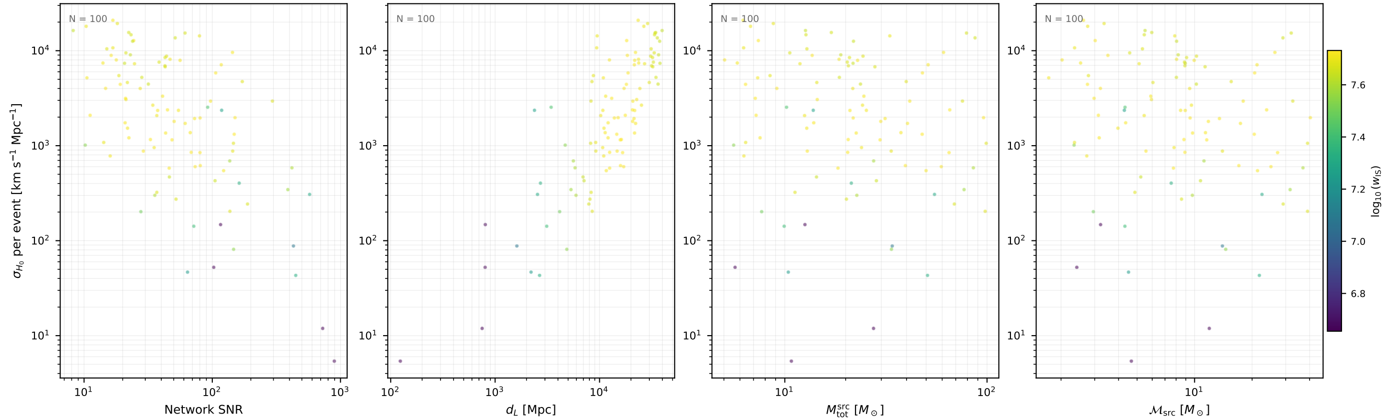
Fisher \sigma_{H_0} per event CE / var03 (100 events, 10 seed(s))
