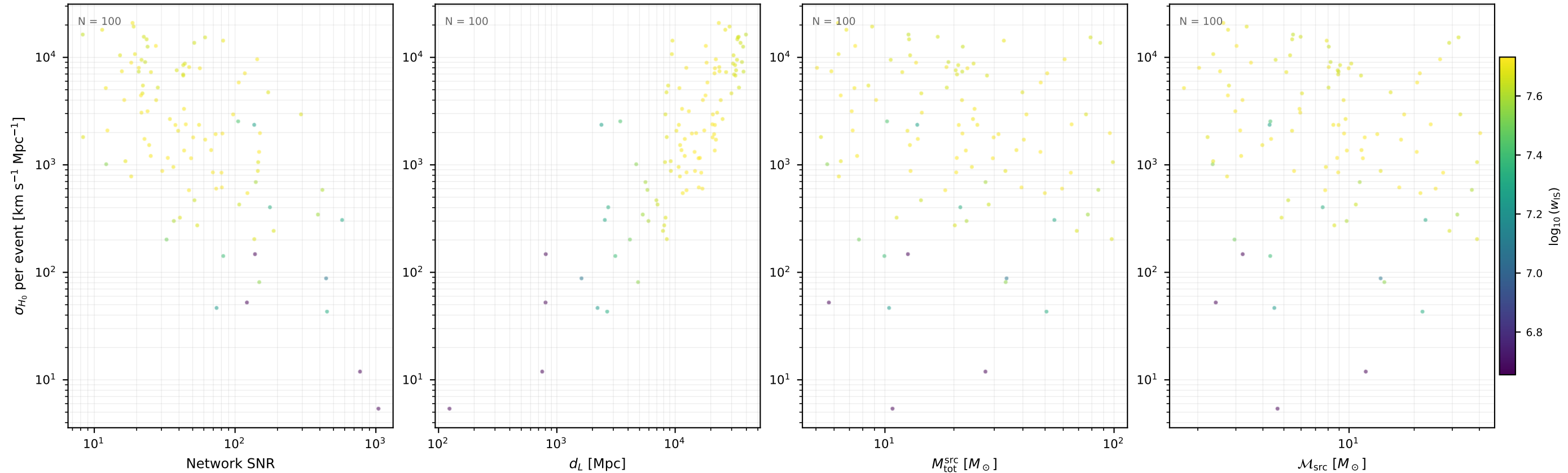
Fisher \sigma_{H_0} per event CE / var02 (100 events, 10 seed(s))
