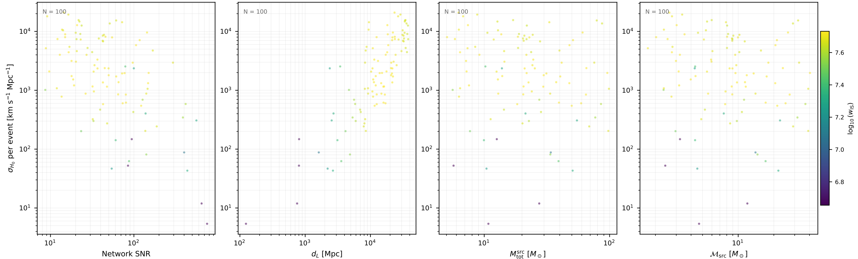
Fisher \sigma_{H_0} per event CE / var01 (100 events, 10 seed(s))
