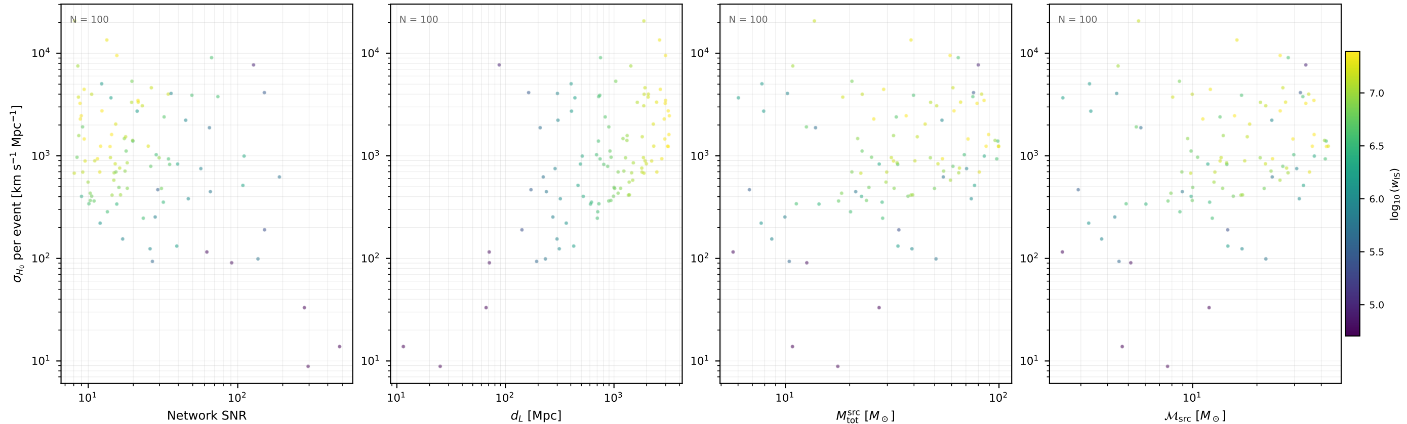
Fisher \sigma_{H_0} per event aLIGO_HLV / var07 (100 events, 10 seed(s))
