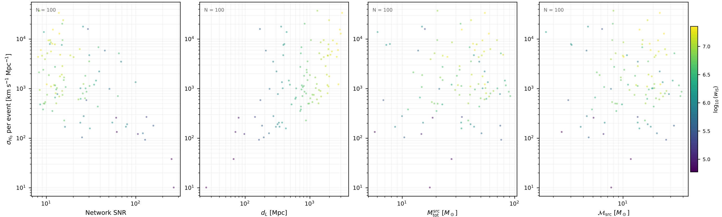
Fisher \sigma_{H_0} per event aLIGO_HLV / var04 (100 events, 10 seed(s))
