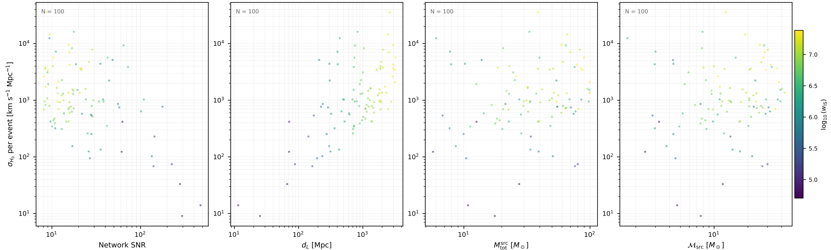
Fisher \sigma_{H_0} per event aLIGO_HLV / baseline (100 events, 10 seed(s))
