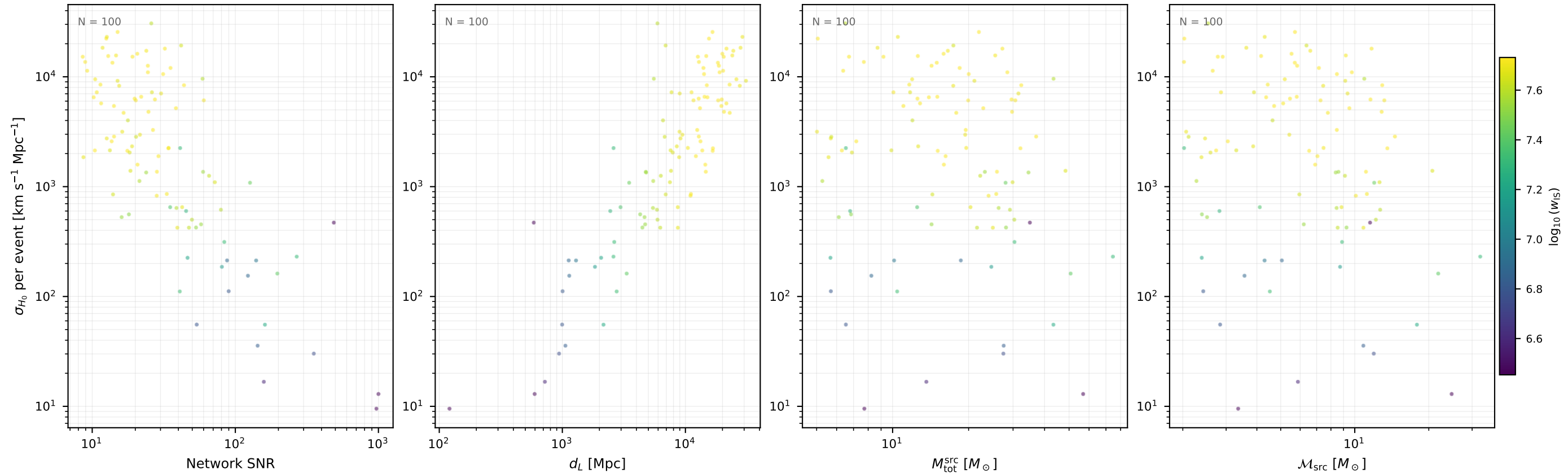
Fisher \sigma_{H_0} per event ET_CE / var05 (100 events, 10 seed(s))
