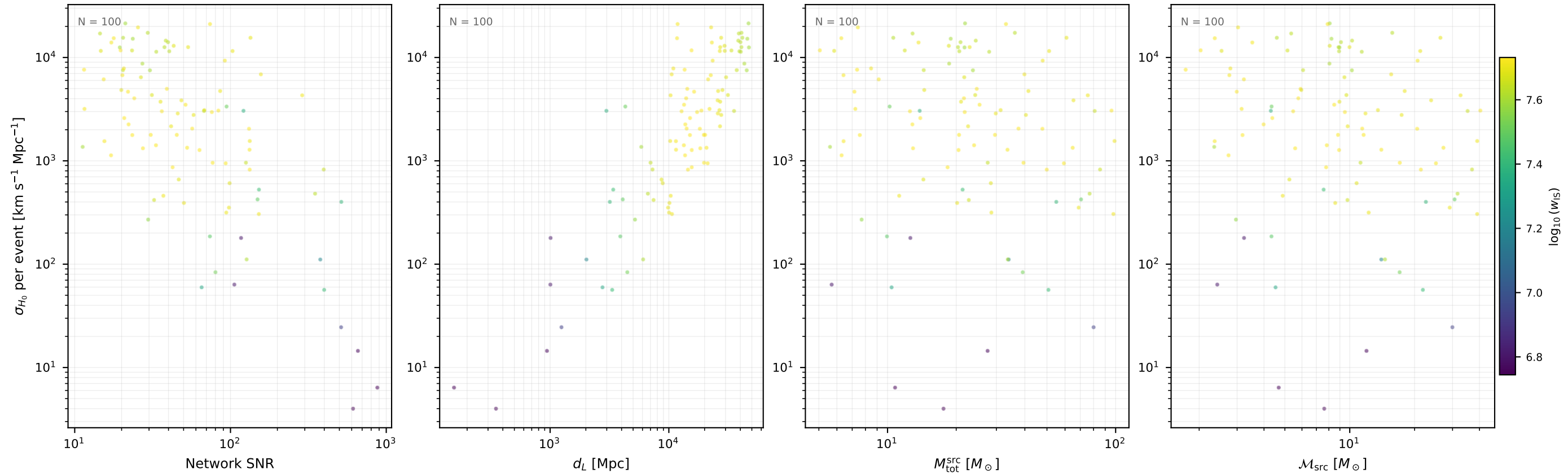
Fisher \sigma_{H_0} per event ET_CE / var02 (100 events, 10 seed(s))
