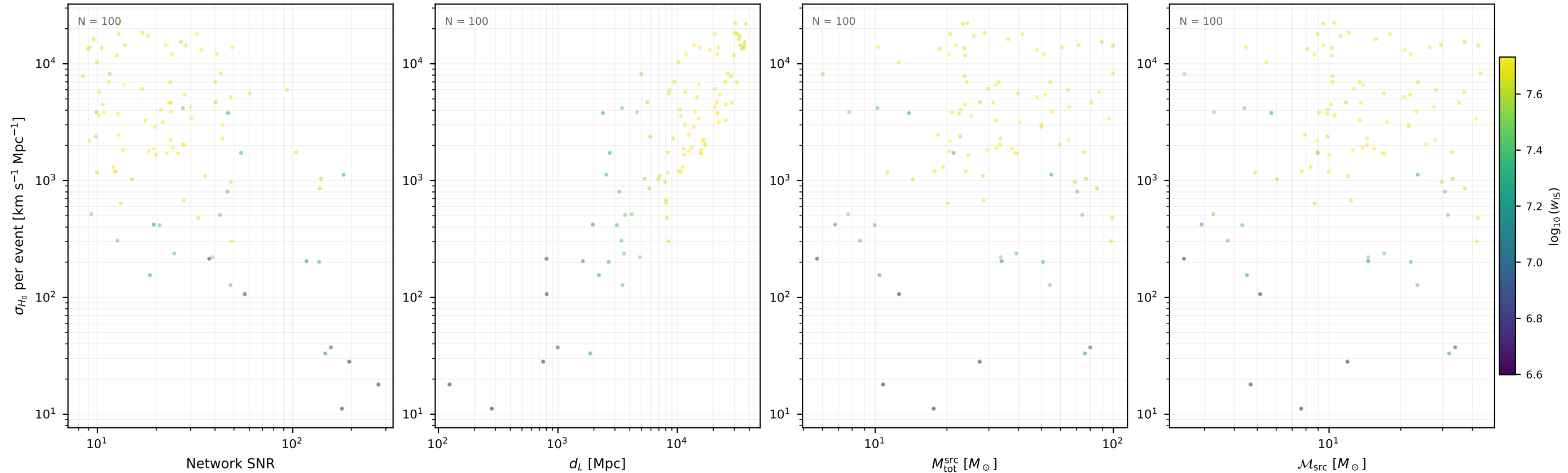
Fisher \sigma_{H_0} per event ET / var08 (100 events, 10 seed(s))
