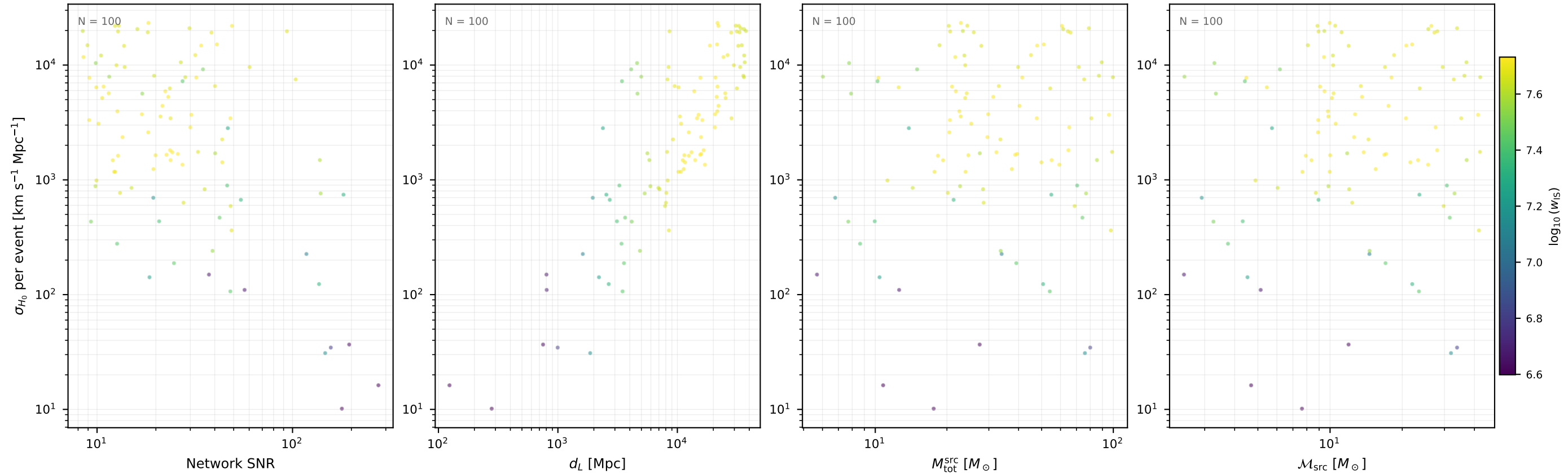
Fisher \sigma_{H_0} per event ET / var07 (100 events, 10 seed(s))
