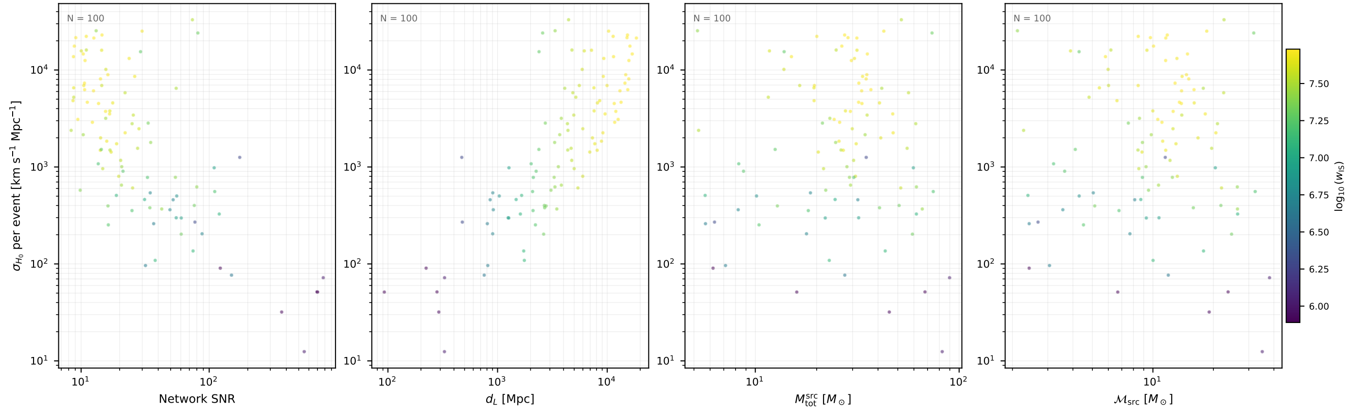
Fisher \sigma_{H_0} per event ET / var05 (100 events, 10 seed(s))
