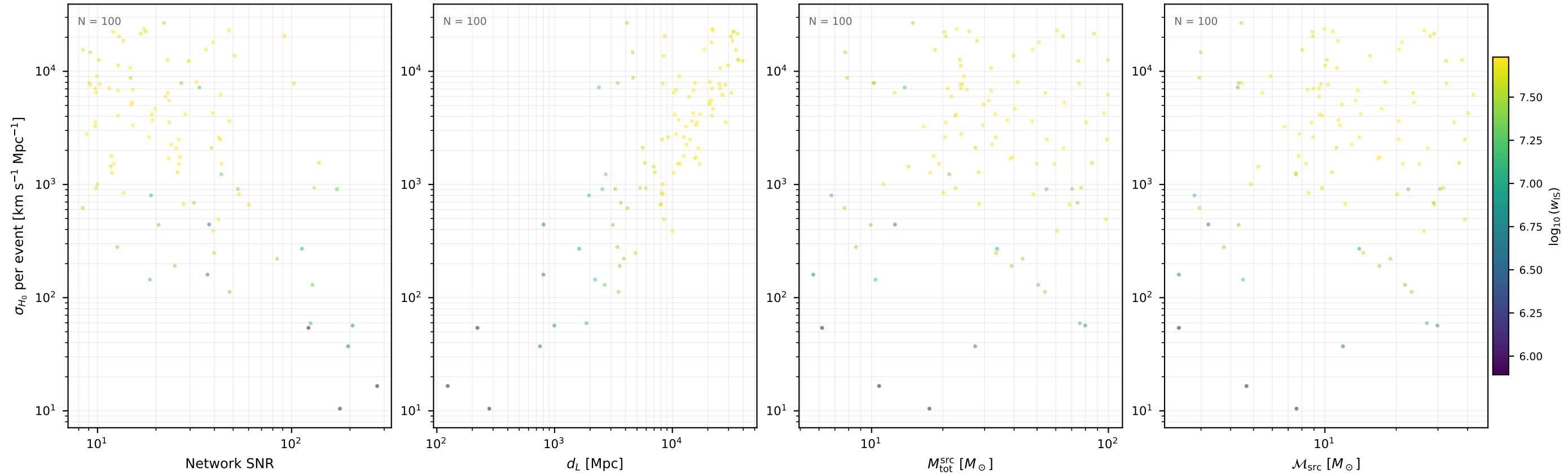
Fisher \sigma_{H_0} per event ET / var03 (100 events, 10 seed(s))
