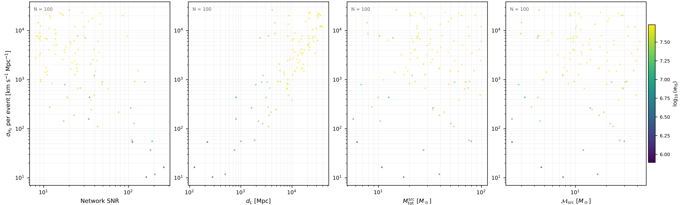
Fisher \sigma_{H_0} per event ET / var01 (100 events, 10 seed(s))
