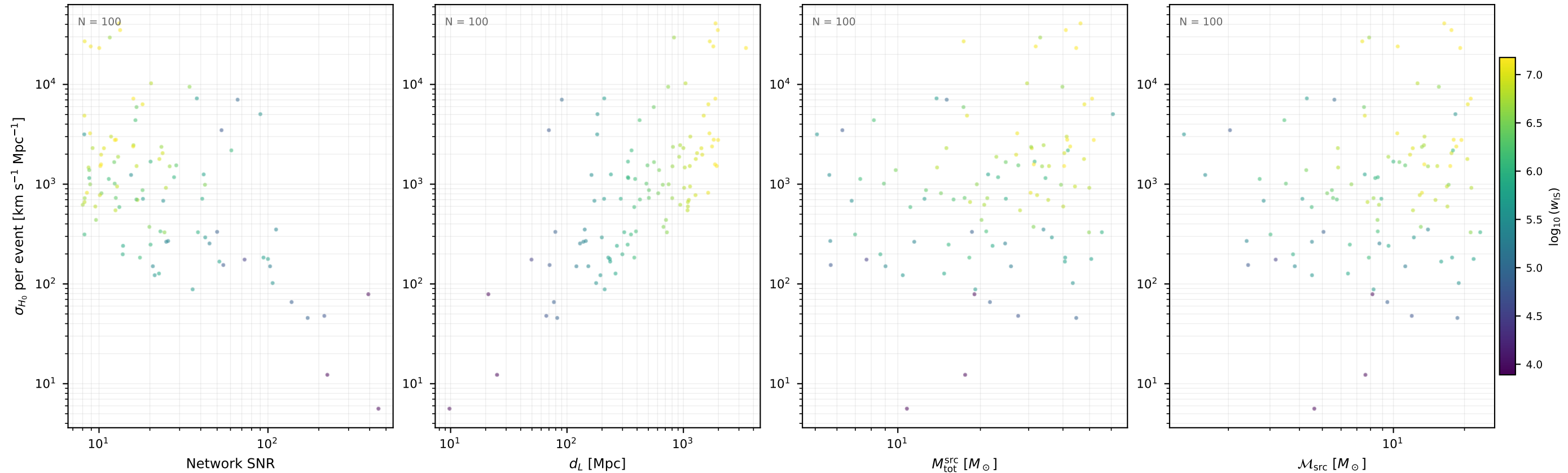
Fisher \sigma_{H_0} per event aLIGO_HLV / var05 (100 events, 10 seed(s))
