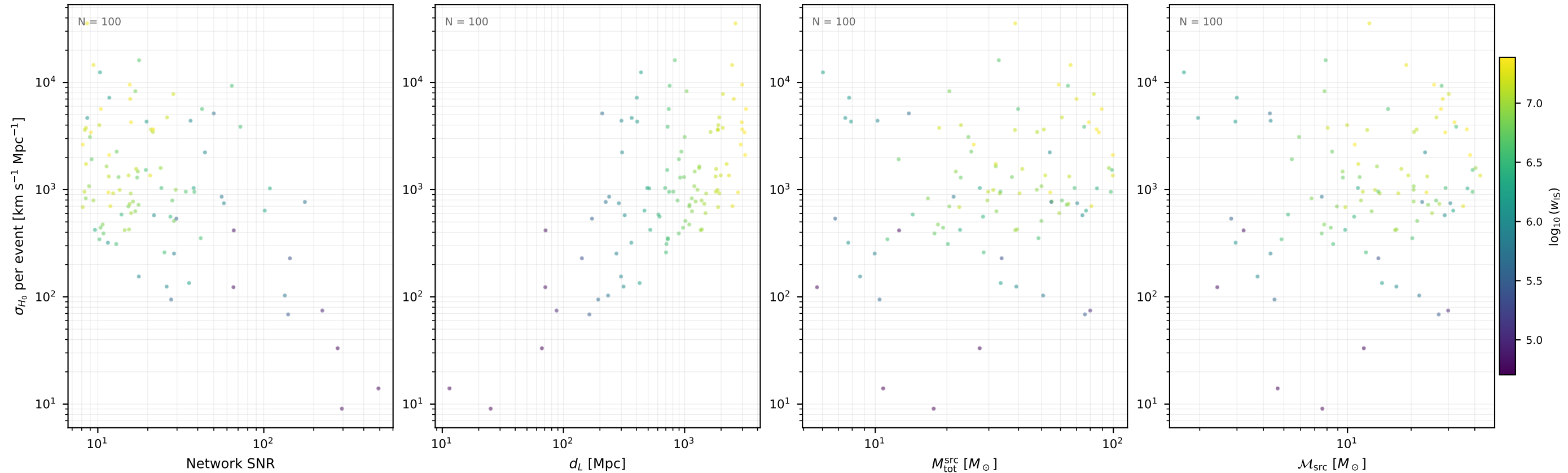
Fisher \sigma_{H_0} per event aLIGO_HLV / var02 (100 events, 10 seed(s))
