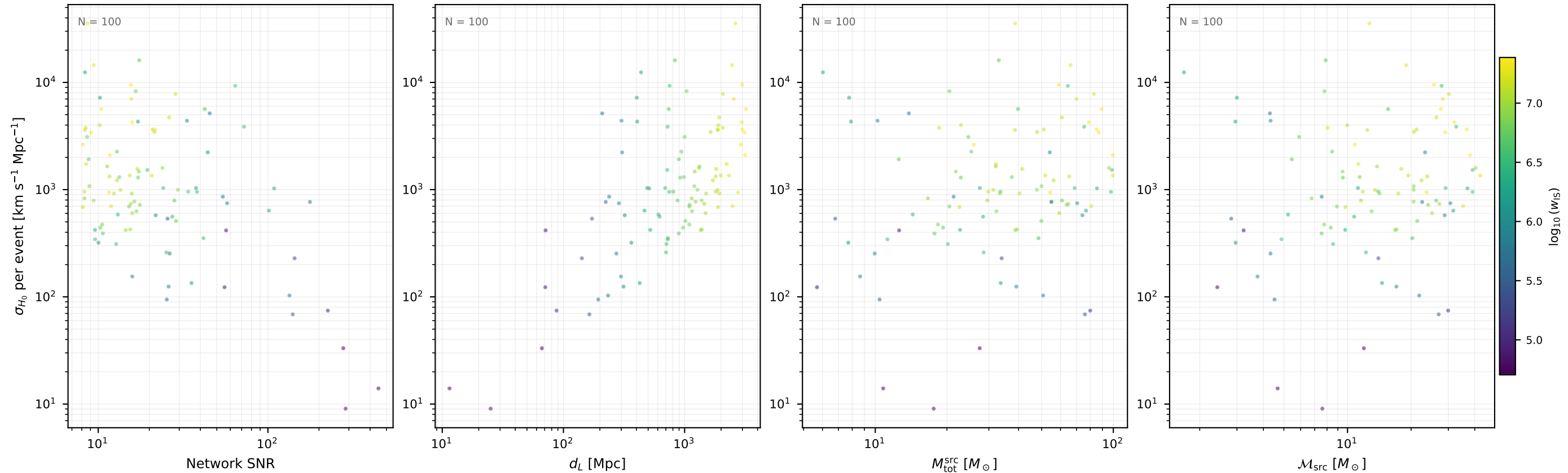
Fisher \sigma_{H_0} per event aLIGO_HLV / var01 (100 events, 10 seed(s))
