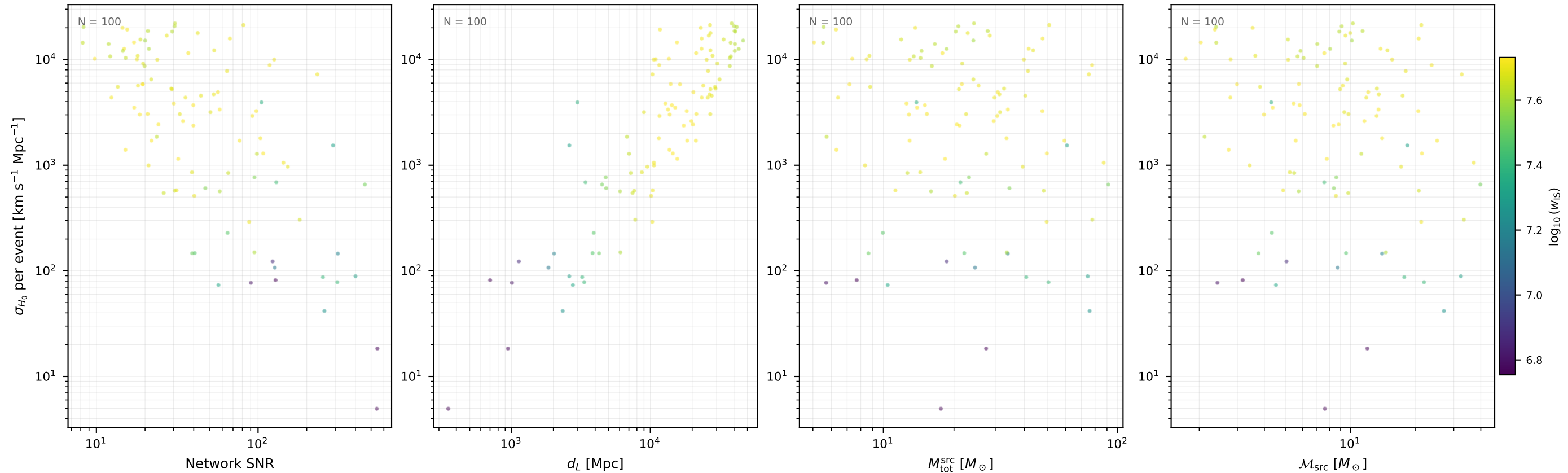
Fisher \sigma_{H_0} per event ET_CE / var04 (100 events, 10 seed(s))
