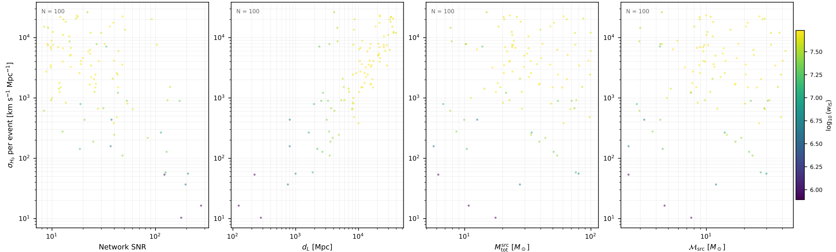
Fisher \sigma_{H_0} per event ET / baseline (100 events, 10 seed(s))
