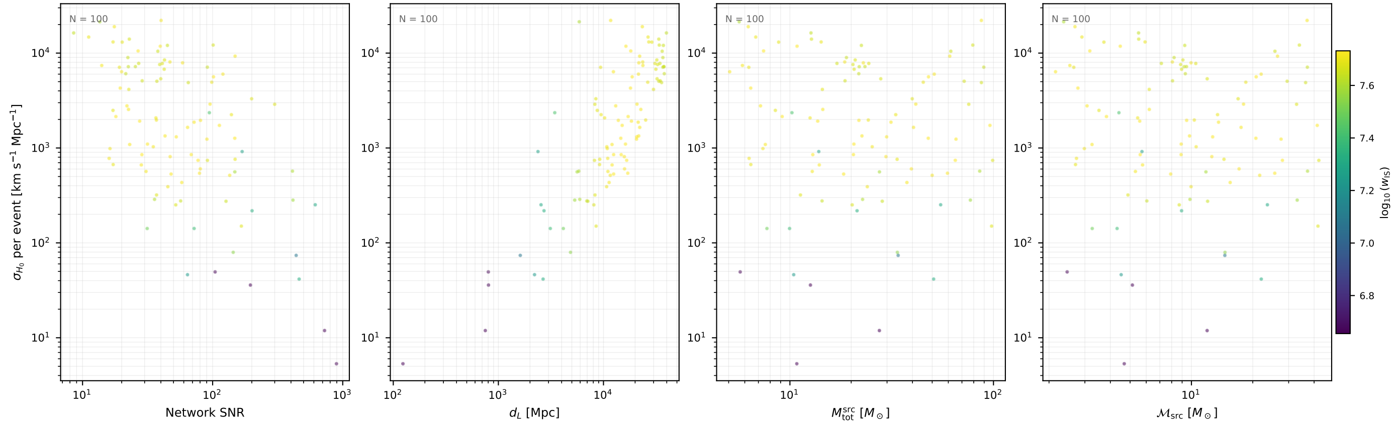
Fisher \sigma_{H_0} per event CE / var07 (100 events, 10 seed(s))
