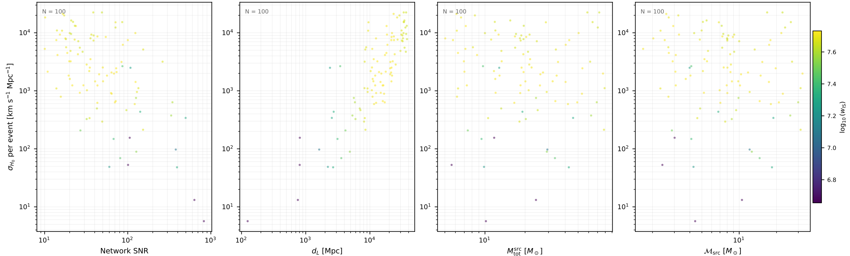
Fisher \sigma_{H_0} per event CE / var06 (100 events, 10 seed(s))
