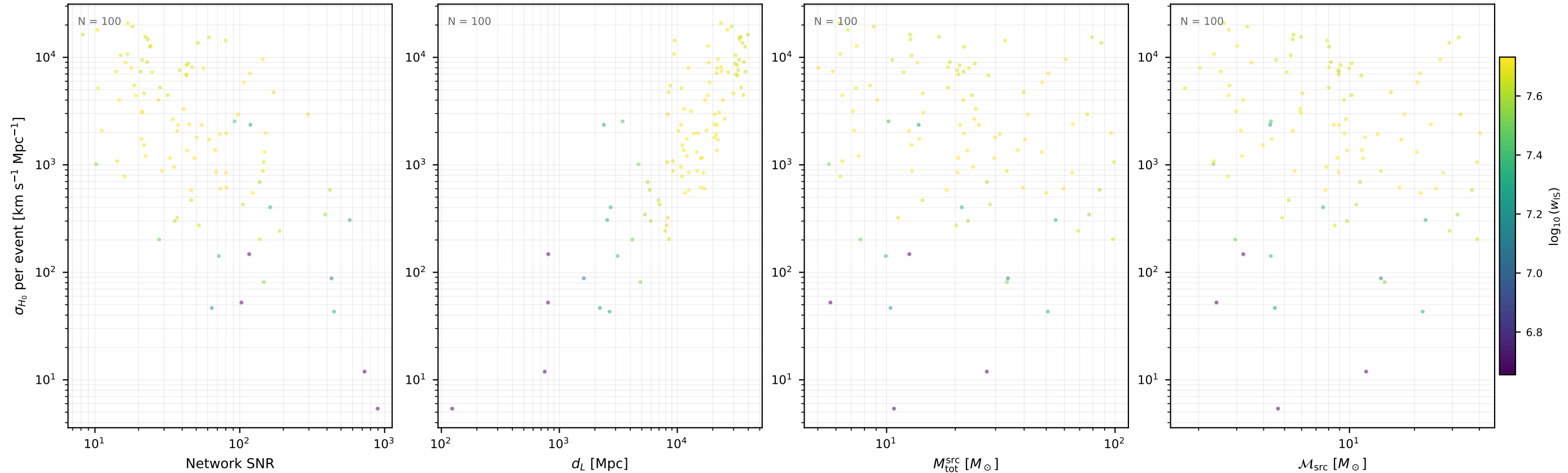
Fisher \sigma_{H_0} per event CE / baseline (100 events, 10 seed(s))
