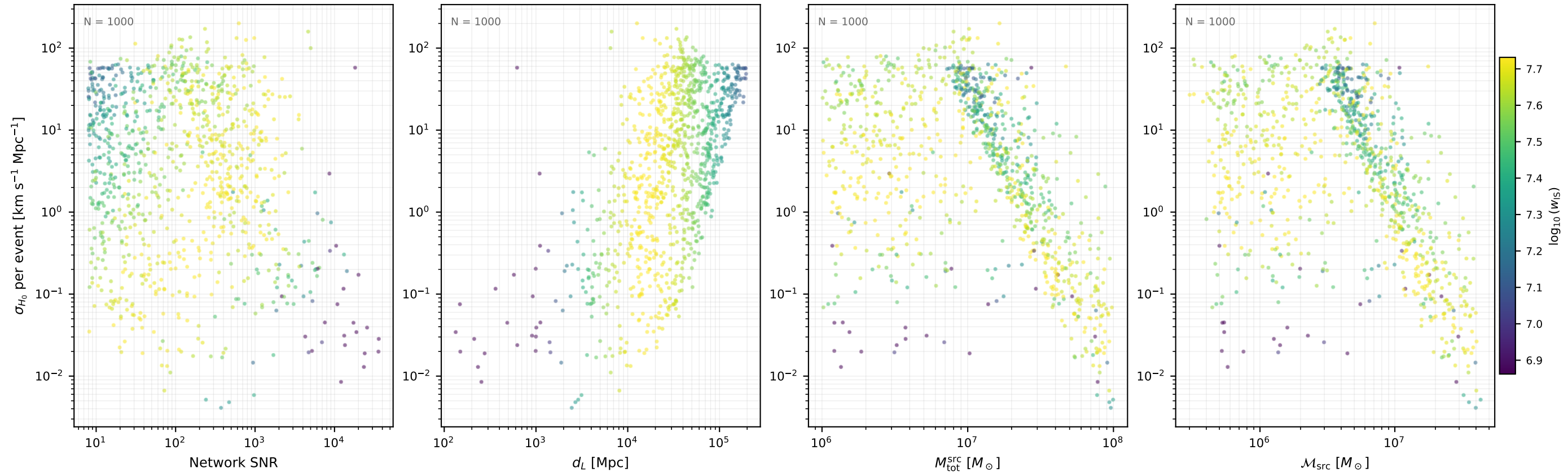
Fisher \sigma_{H_0} per event LISA n_samples=4096 (1000 events, 10 seed(s))
