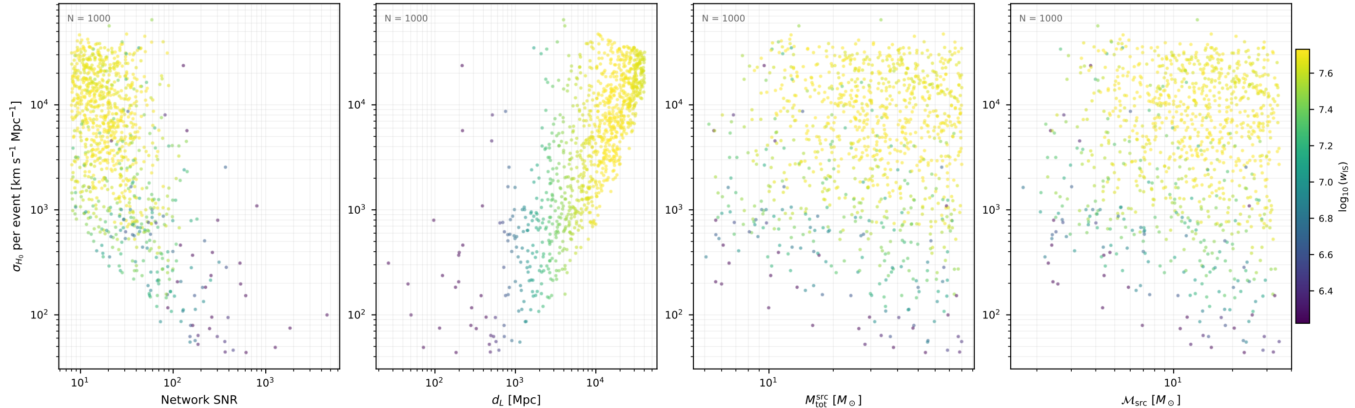
Fisher \sigma_{H_0} per event ET / var06 (1000 events, 10 seed(s))
