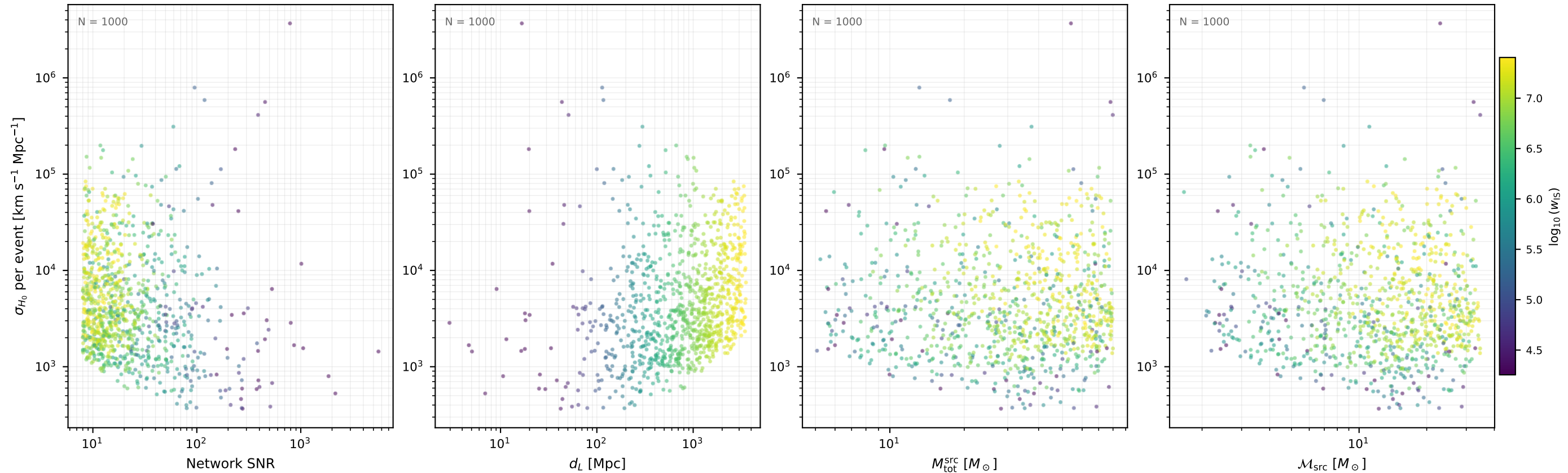
Fisher \sigma_{H_0} per event aLIGO_HLV / var06 (1000 events, 10 seed(s))
