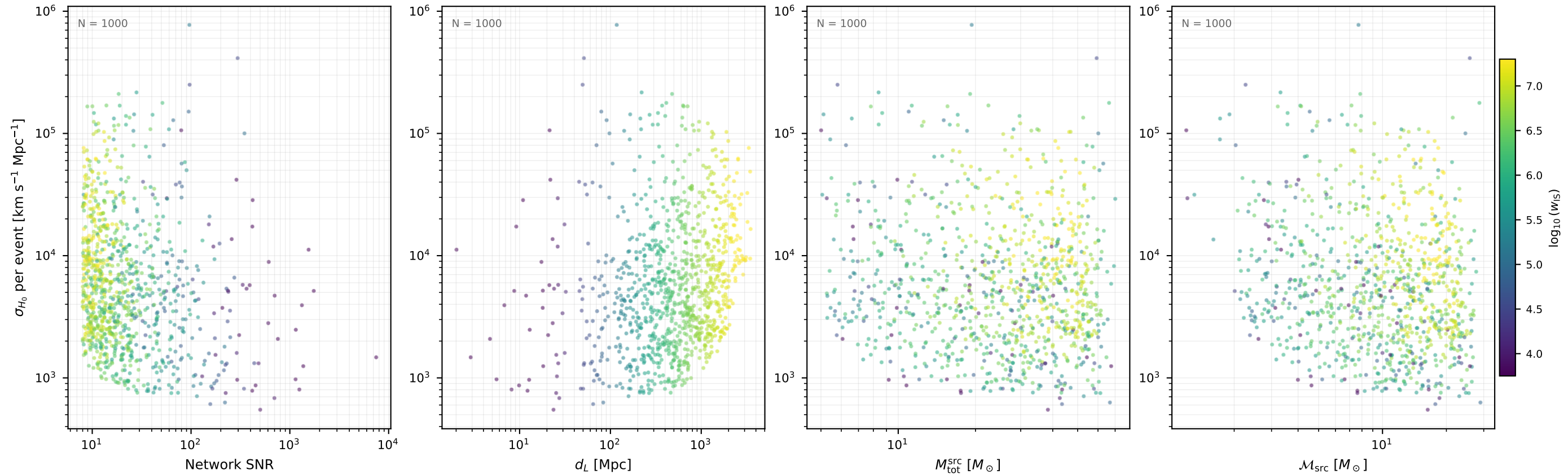
Fisher \sigma_{H_0} per event aLIGO_HLV / var05 (1000 events, 10 seed(s))
