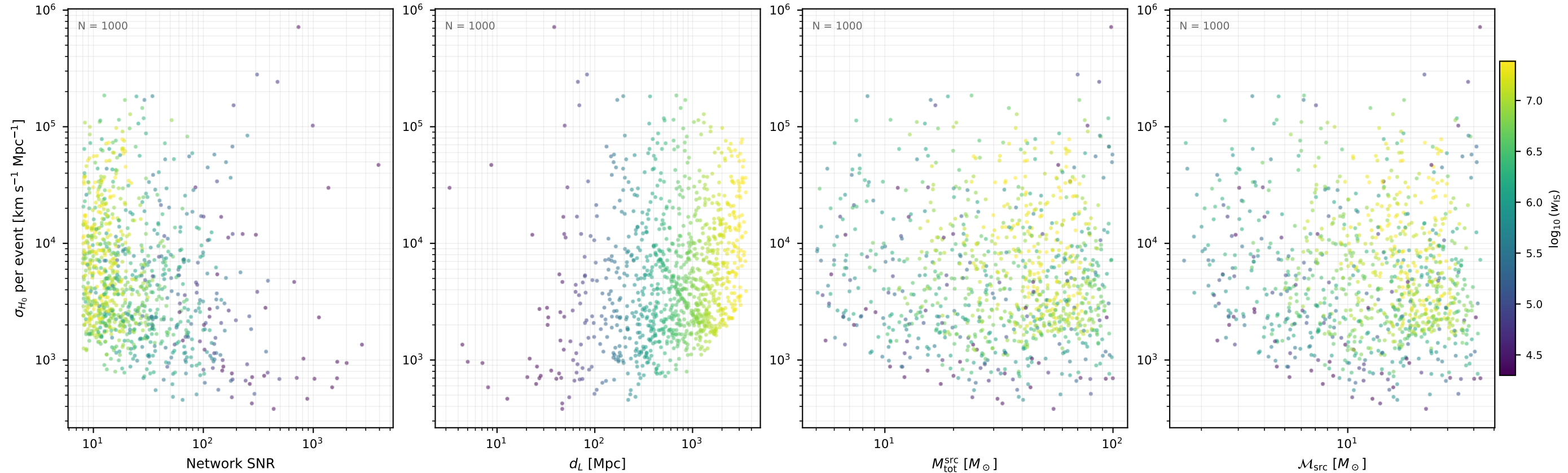
Fisher \sigma_{H_0} per event aLIGO_HLV / var04 (1000 events, 10 seed(s))
