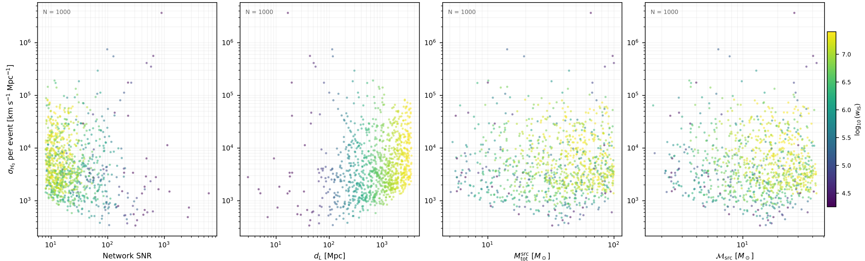
Fisher \sigma_{H_0} per event aLIGO_HLV / var01 (1000 events, 10 seed(s))
