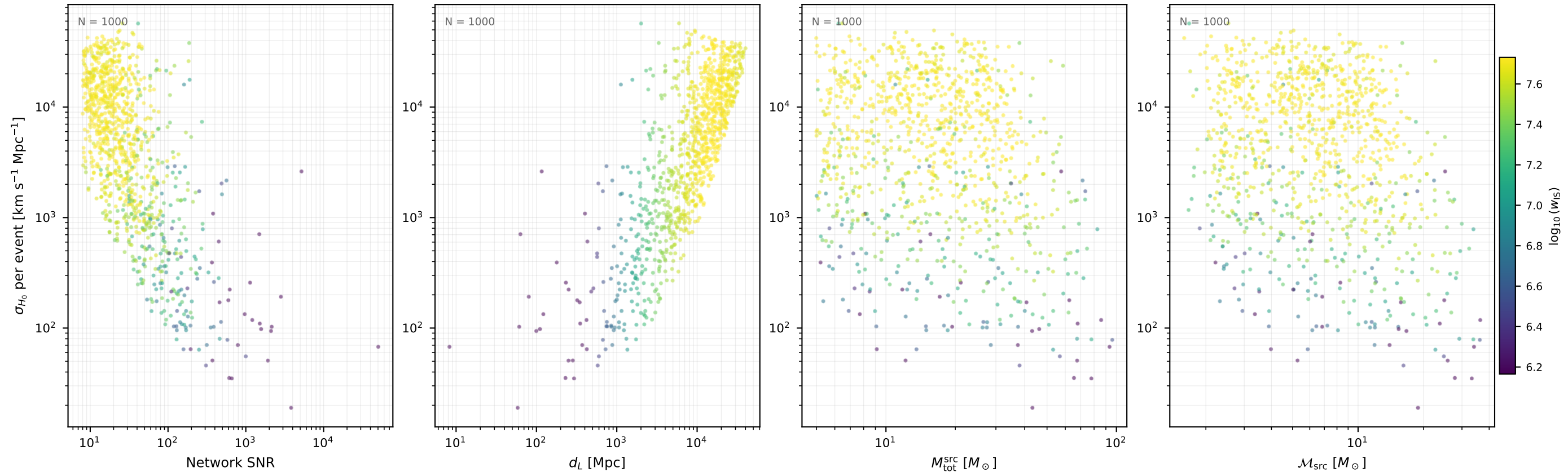
Fisher \sigma_{H_0} per event ET_CE / var05 (1000 events, 10 seed(s))
