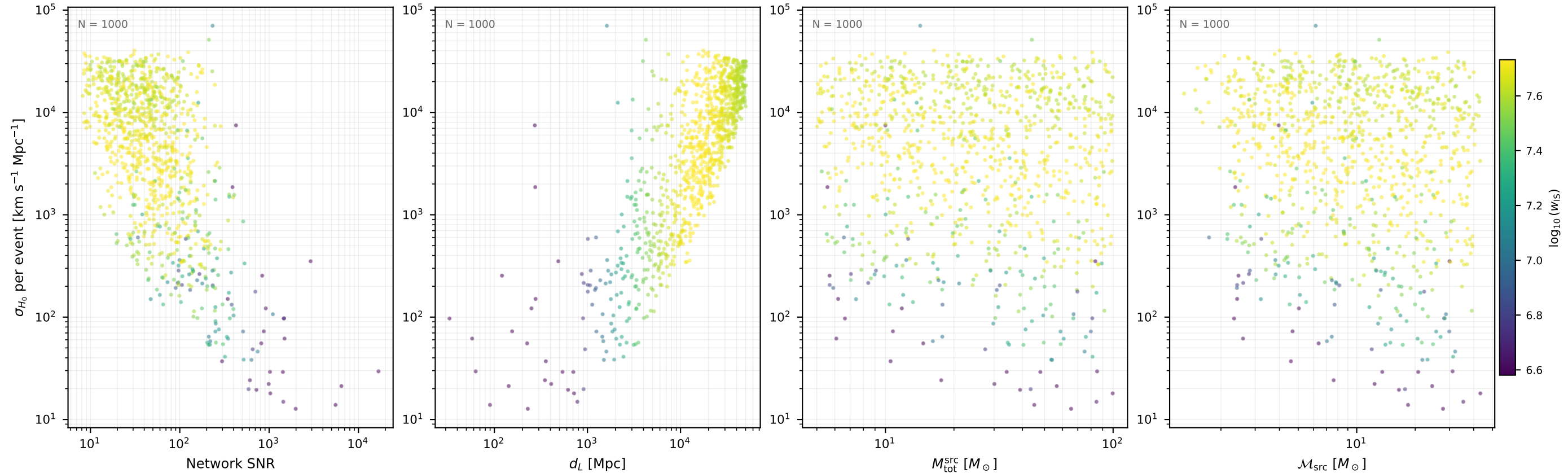
Fisher \sigma_{H_0} per event ET_CE / var02 (1000 events, 10 seed(s))
