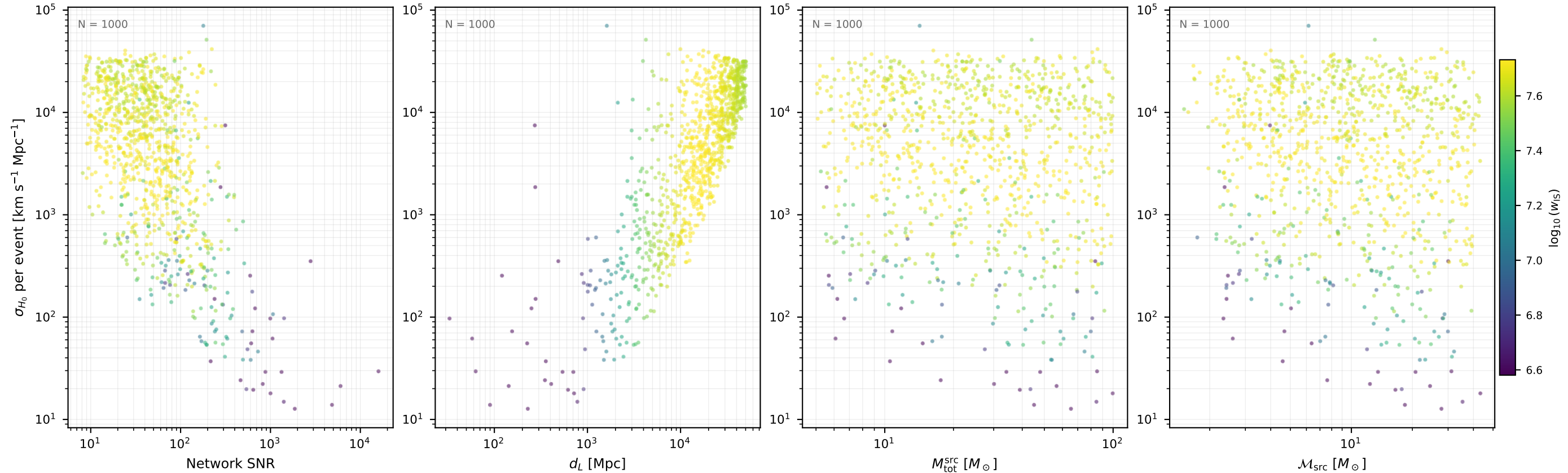
Fisher \sigma_{H_0} per event ET_CE / var01 (1000 events, 10 seed(s))
