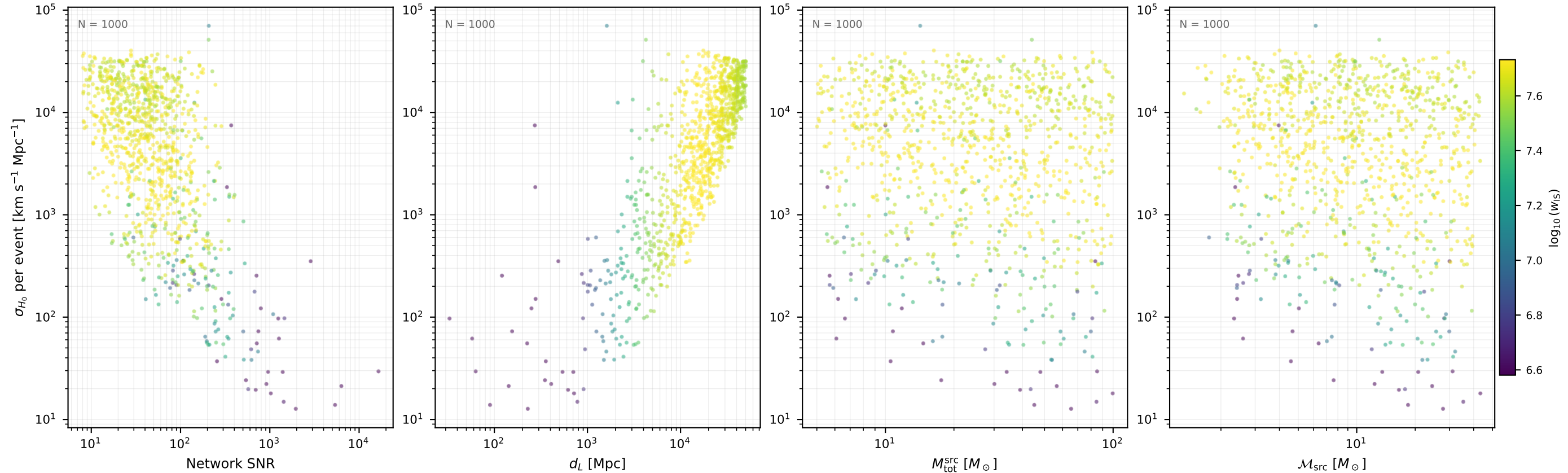
Fisher \sigma_{H_0} per event ET_CE / baseline (1000 events, 10 seed(s))
