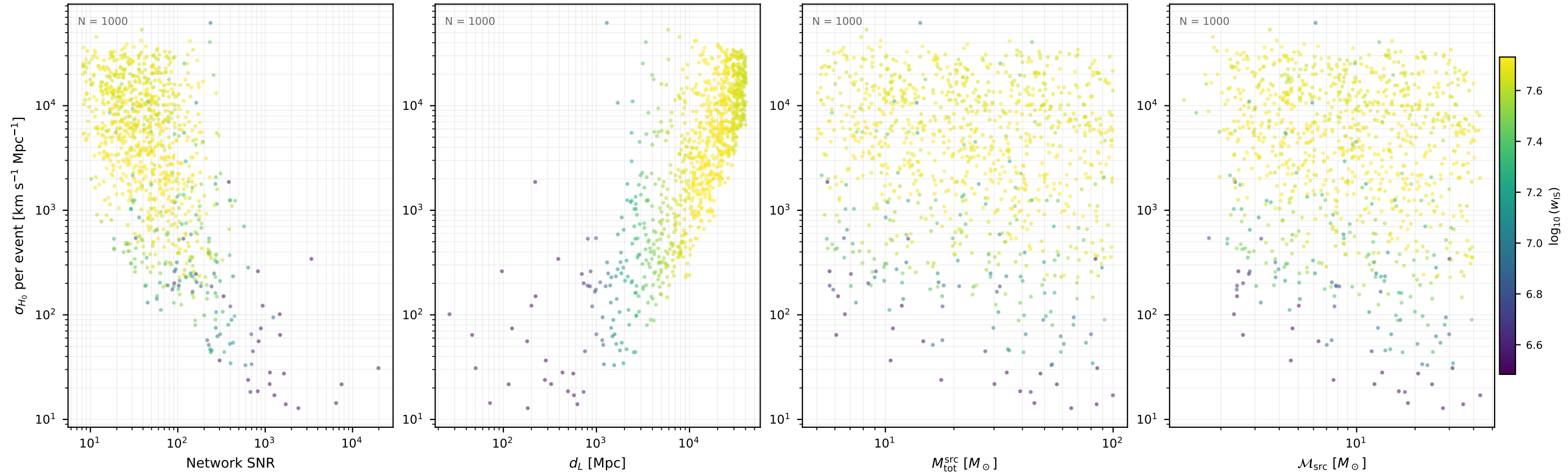
Fisher \sigma_{H_0} per event CE / baseline (1000 events, 10 seed(s))
