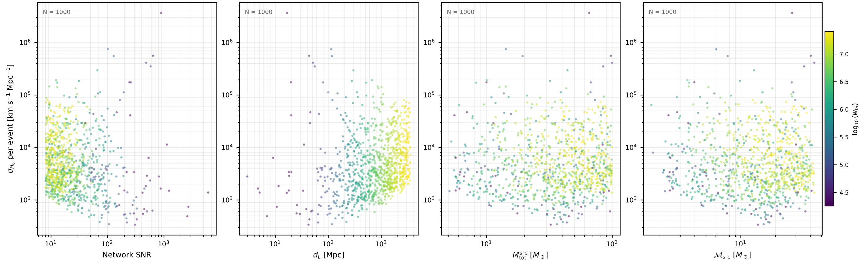
Fisher \sigma_{H_0} per event aLIGO_HLV / var03 (1000 events, 10 seed(s))
