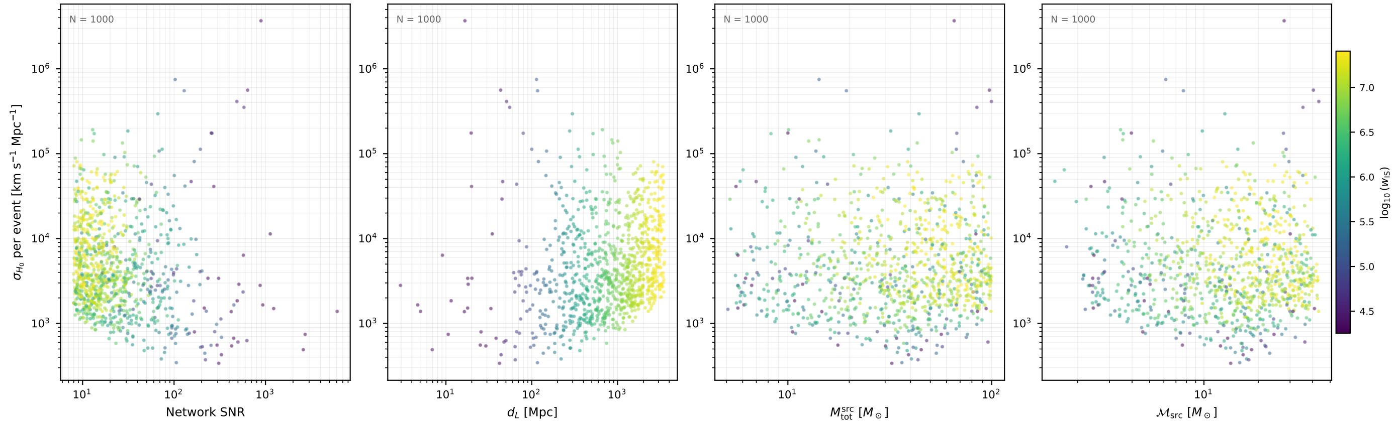
Fisher \sigma_{H_0} per event aLIGO_HLV / var02 (1000 events, 10 seed(s))
